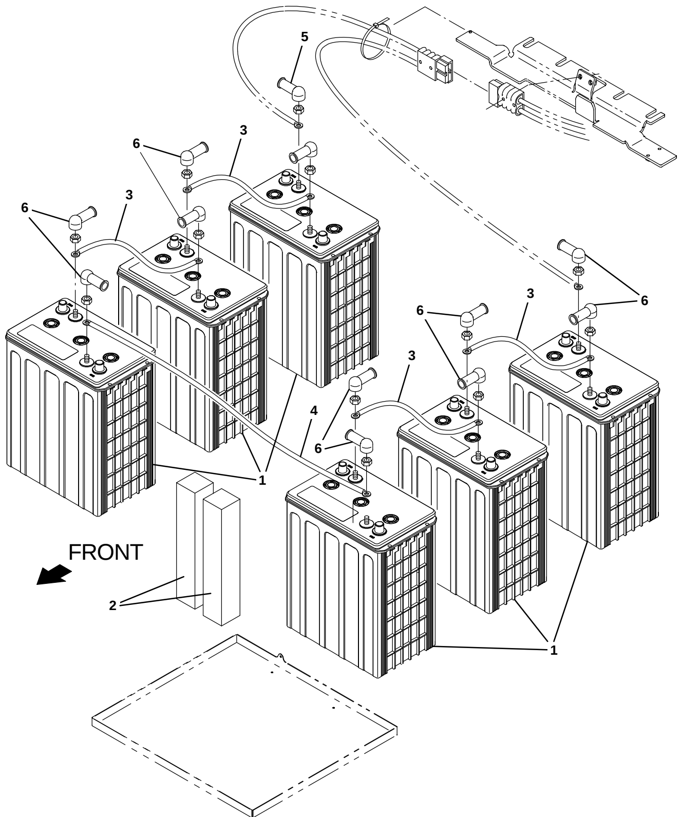
Fig. 23 – Battery Group, 36V 350Ah
