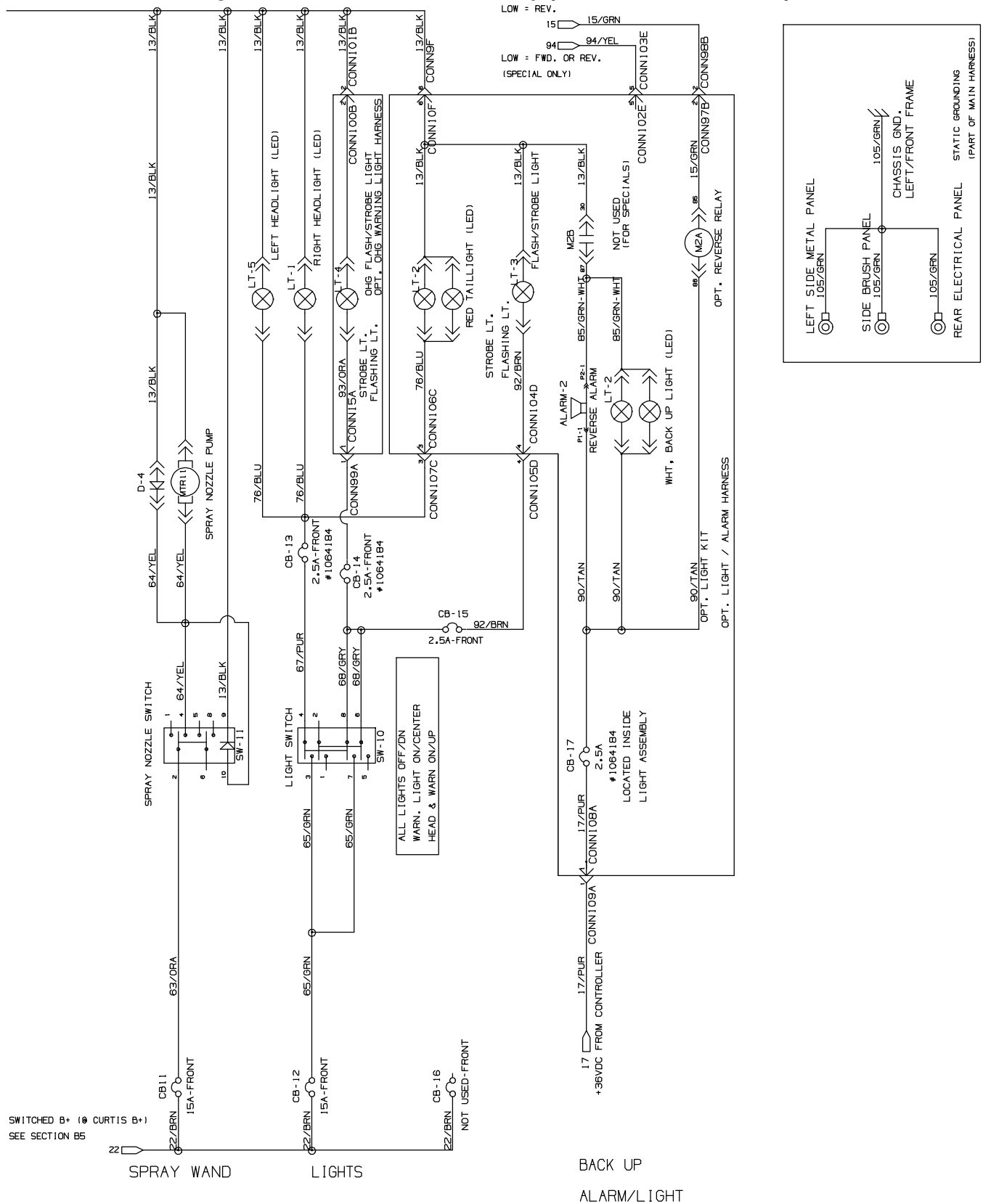
Fig. 25 – Electrical Schematic Group (S/N 10000000–10863997)
