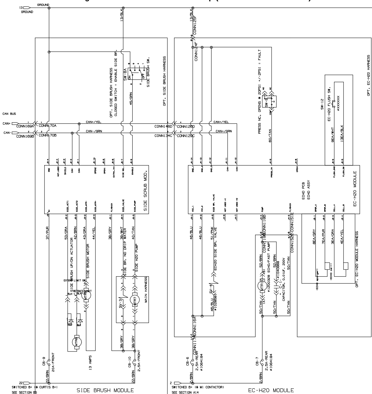
Fig. 25 – Electrical Schematic Group (S/N 10000000–10863997)
