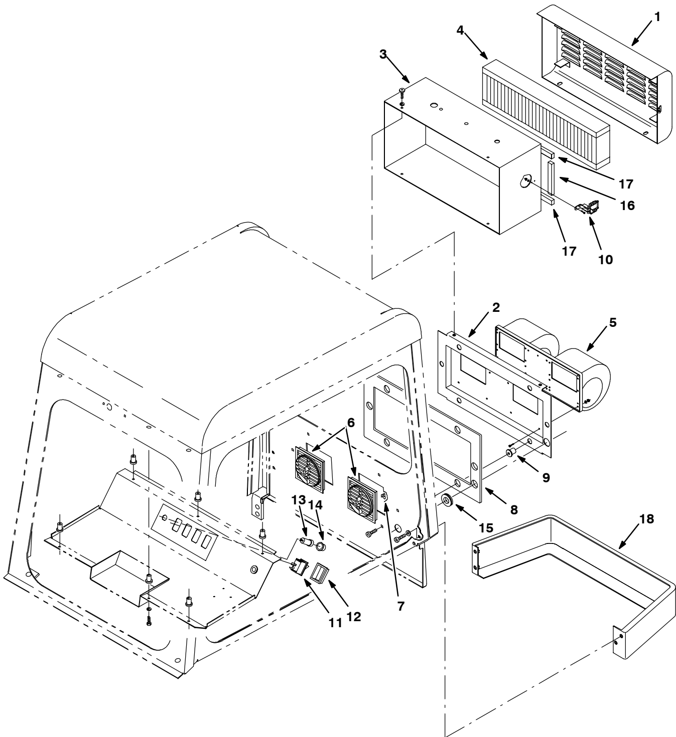
Fig. 16 - Cab Pressurizer Kit (000000-008645)
