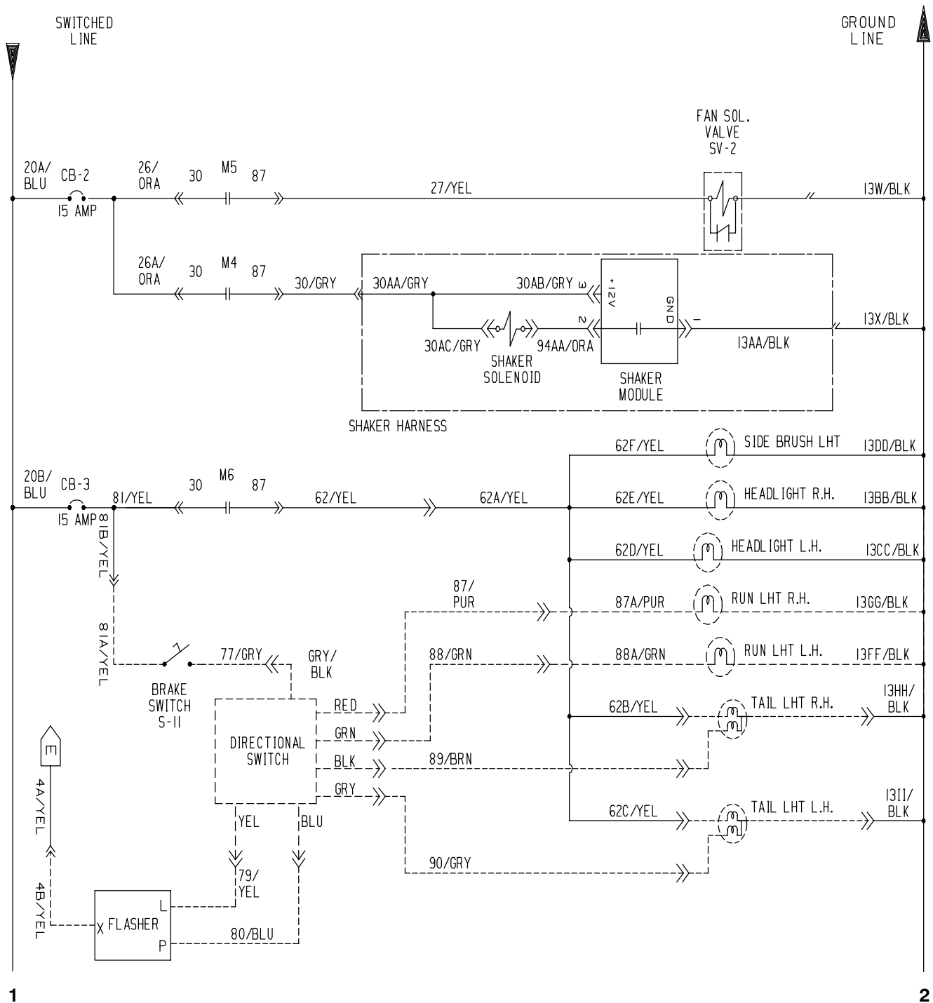
Fig. 55 - Electrical Schematic
