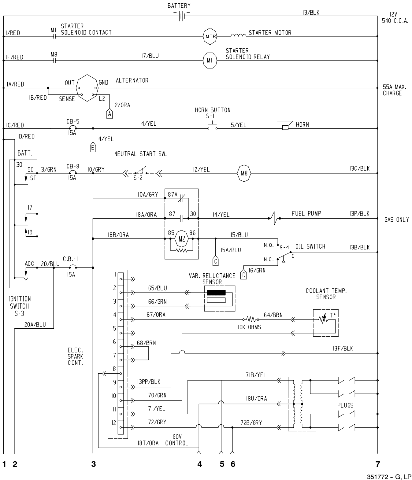
Fig. 55 - Electrical Schematic
