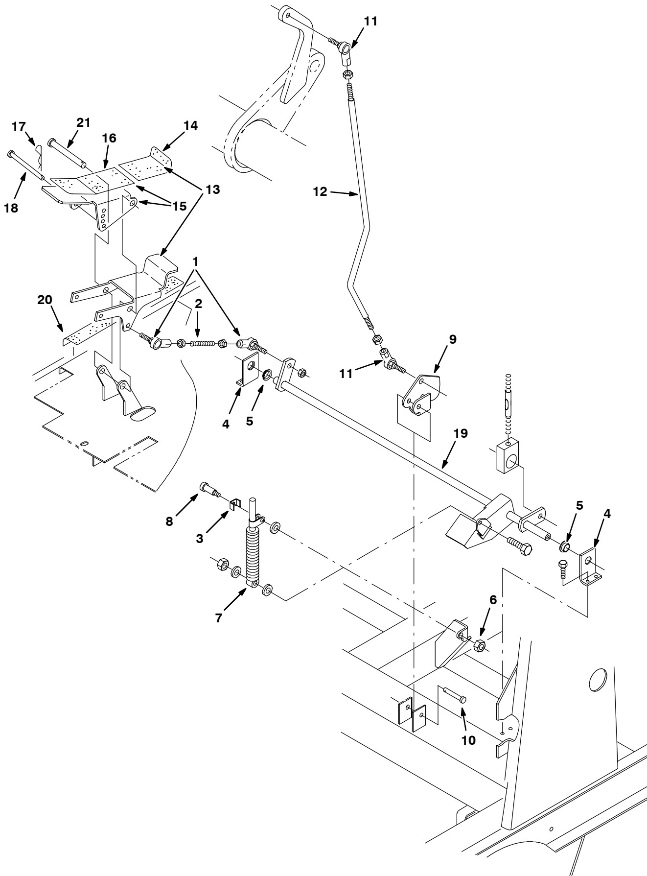
Fig. 34 - Directional Pedal Group
