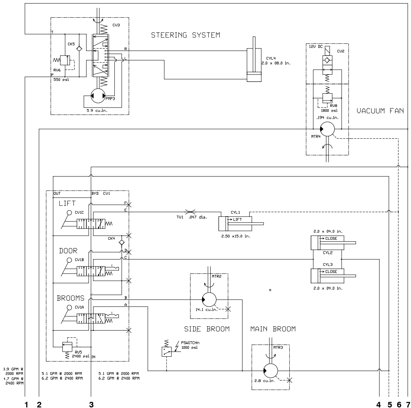
Fig. 48 - Hydraulic Schematic
