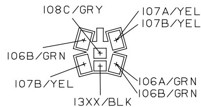
VIEW I-I
