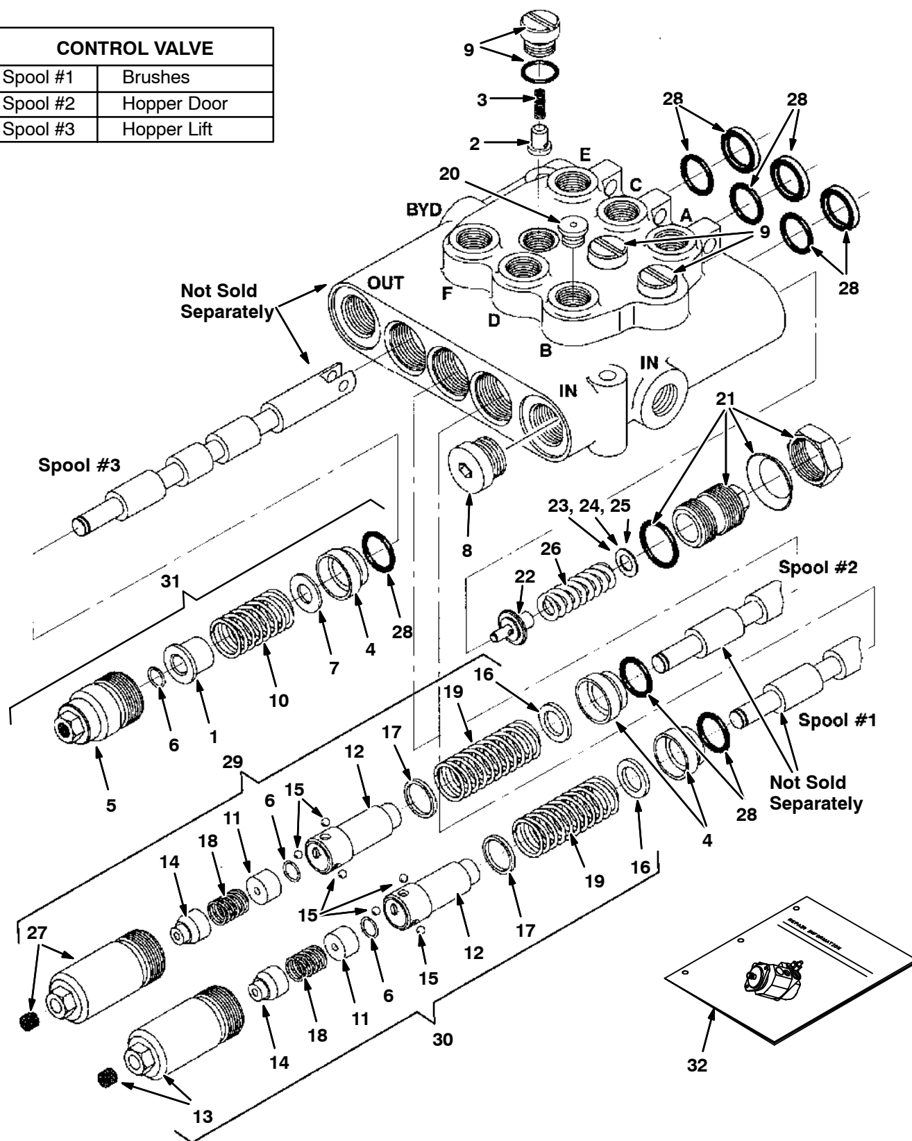
Fig. 12 - Hydraulic Valve Breakdown, 374547
