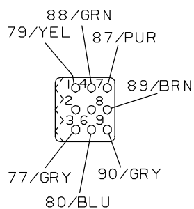
VIEW N-N
