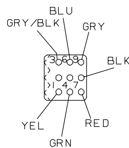
VIEW O-O
