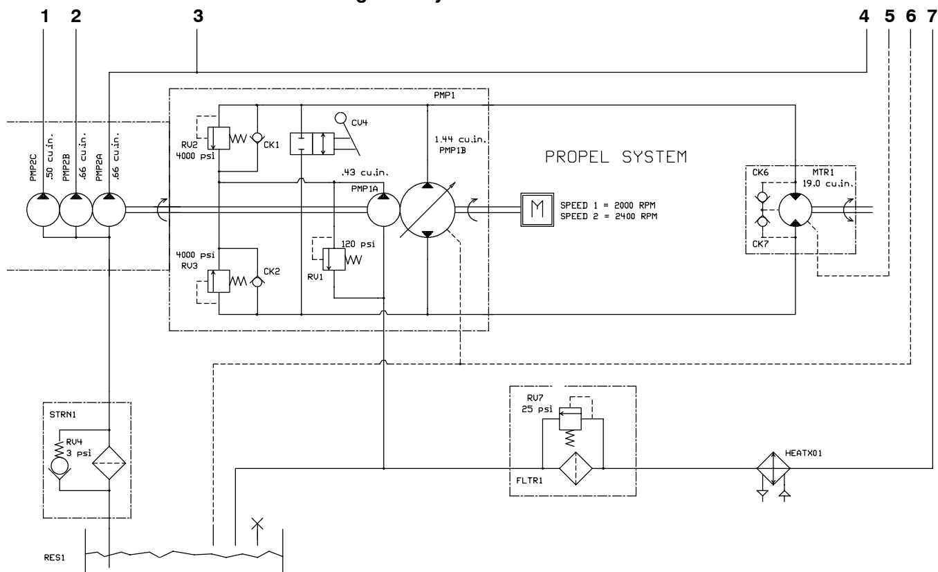
Fig. 48 - Hydraulic Schematic
