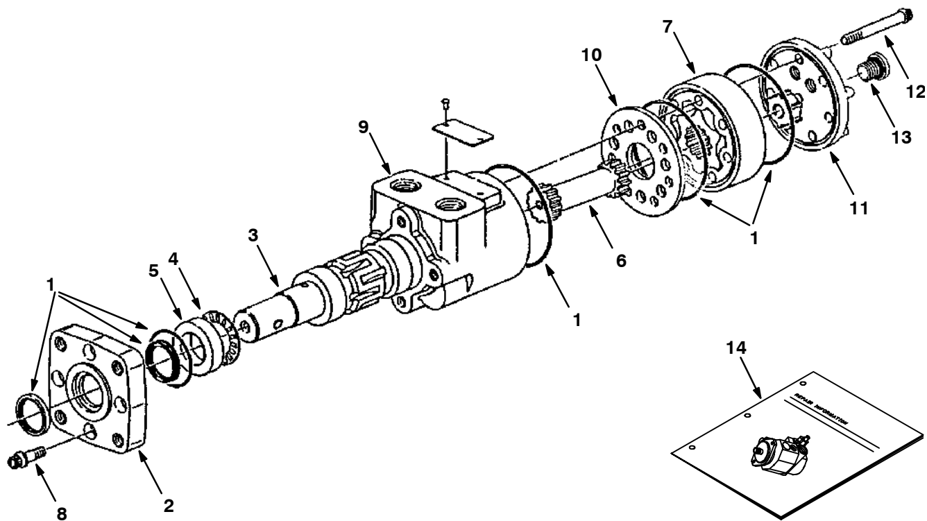
Fig. 10 - Hydraulic Motor Breakdown, 373340
