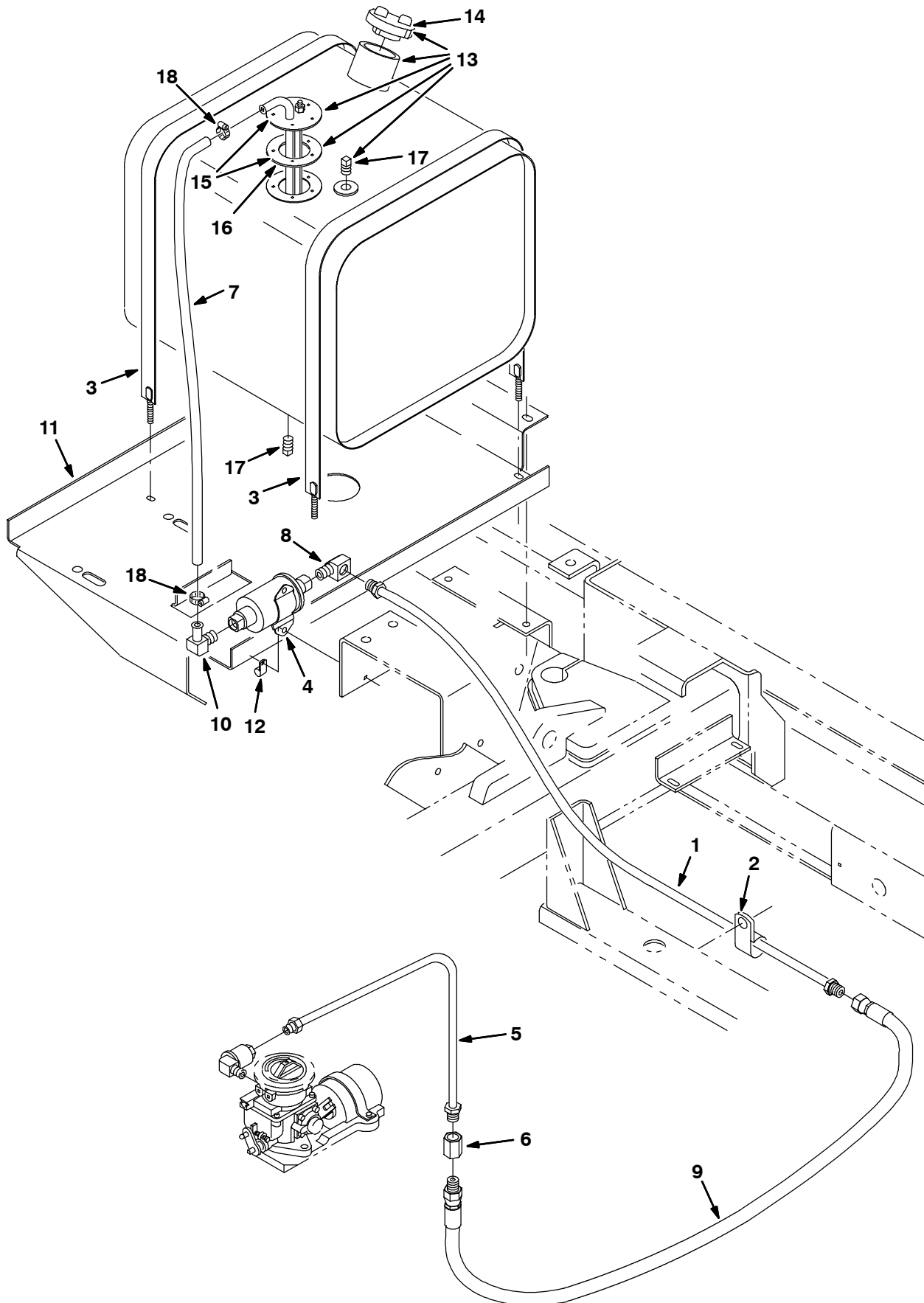
Fig. 25 - Fuel Tank Group, Gasoline
