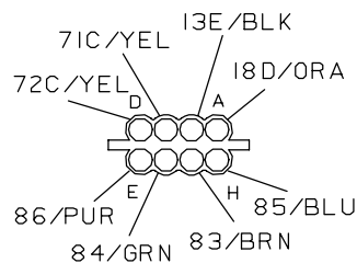
VIEW C-C
