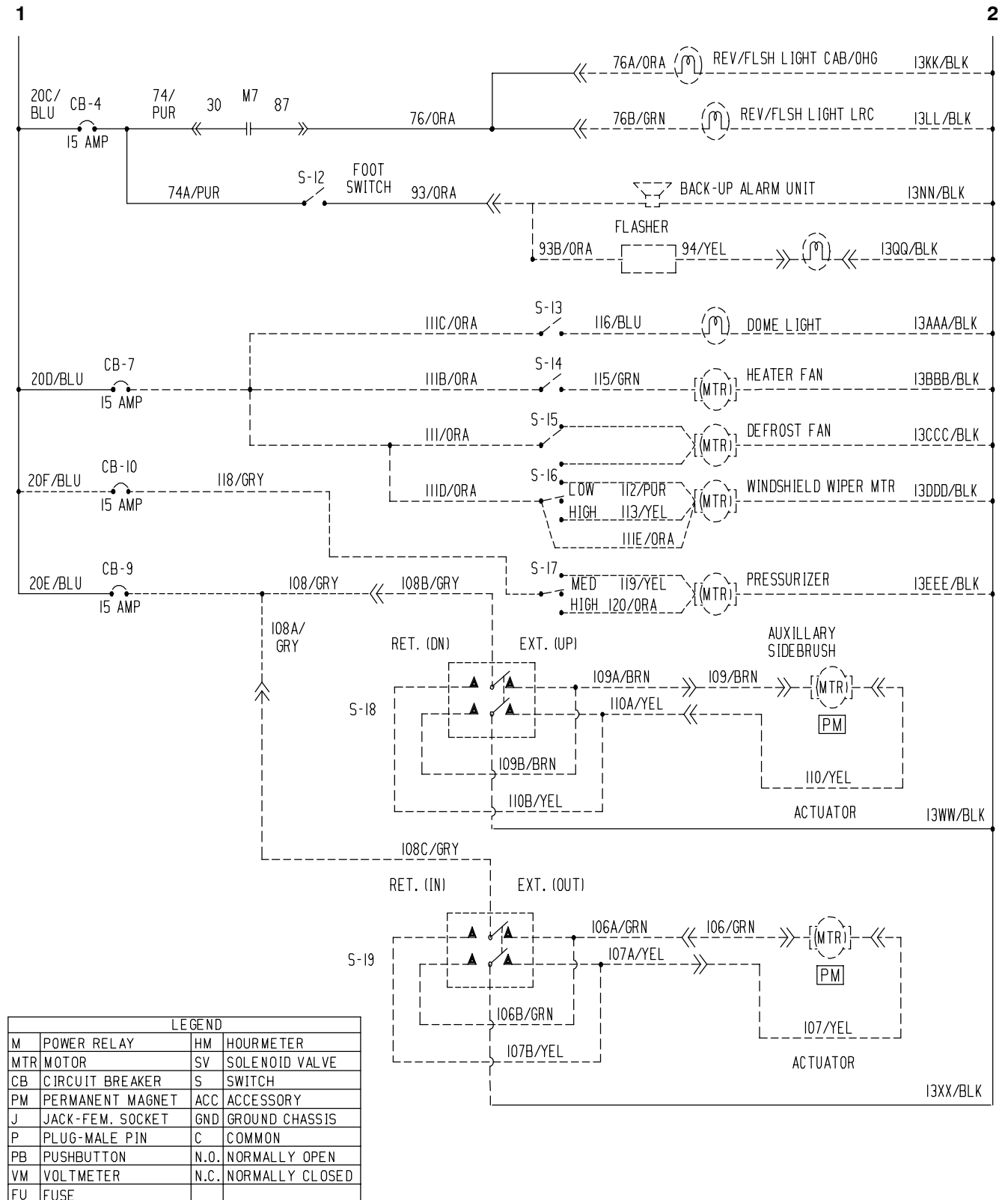
Fig. 55 - Electrical Schematic
