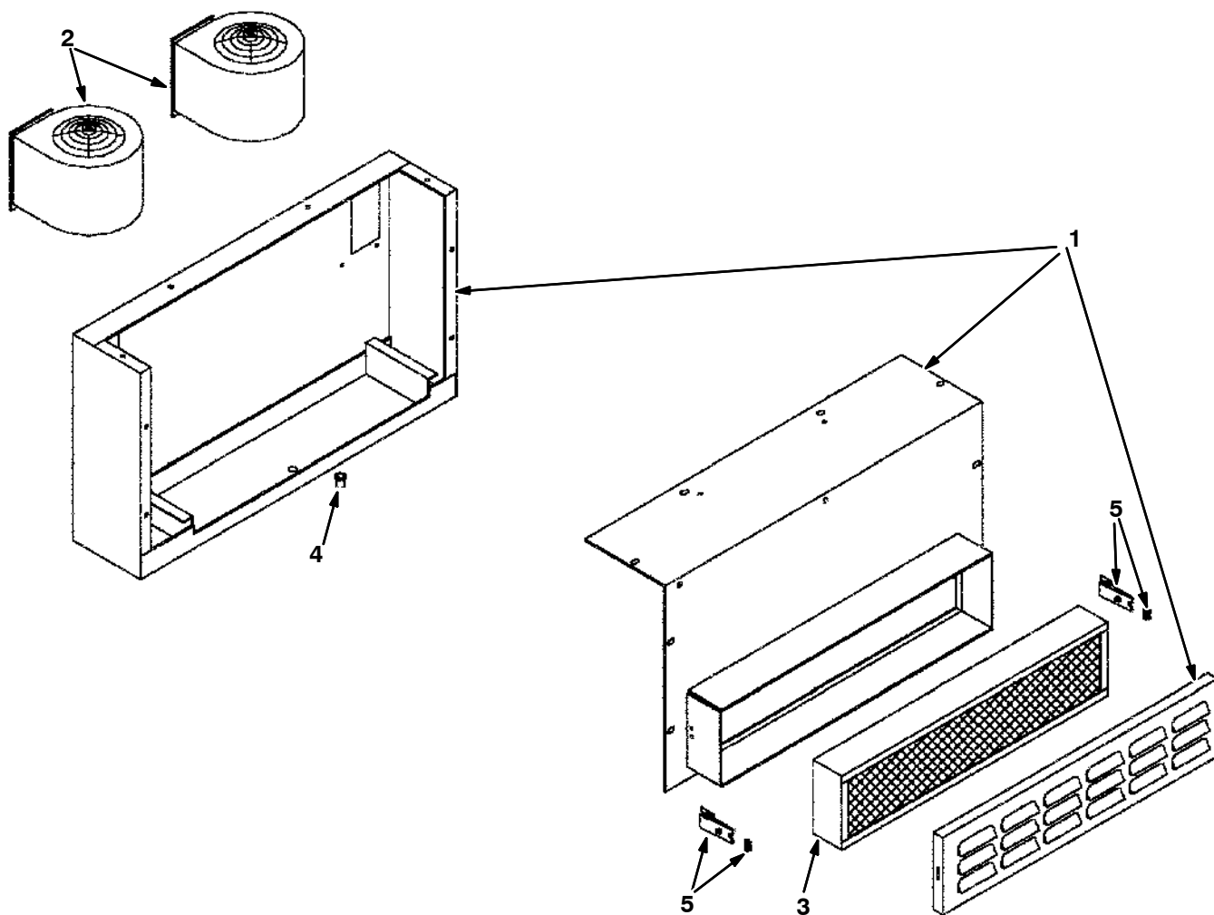
Fig. 19 - Pressurizer Breakdown, 393384
