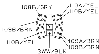
VIEW H-H
