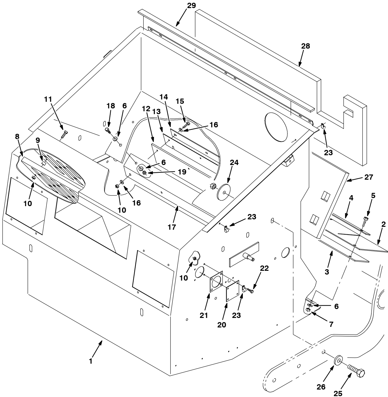
Fig. 36 - Hopper Group
