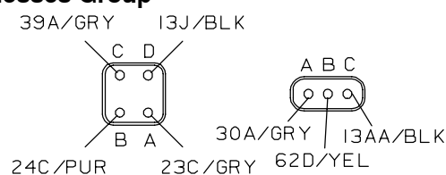
VIEW B-B
