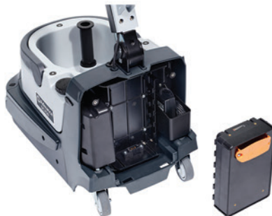
Powered by an easily accessible 36 V lithium battery optimized by BMS (Battery Management System) that monitors and optimizes battery performances, ensuring a safe, efficient energy source with a long life.
