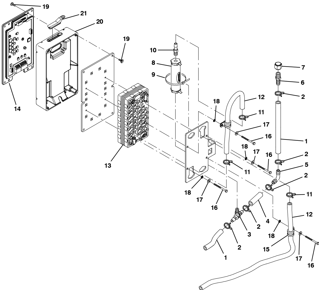
Fig. 14 - ec-H20 Module Assembly Breakdown, 9007882
