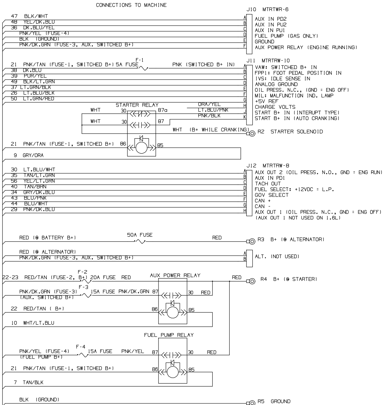
Fig. 74 - Electrical Schematic, Gasoline/LPG Engine Harness (000000-001499)
