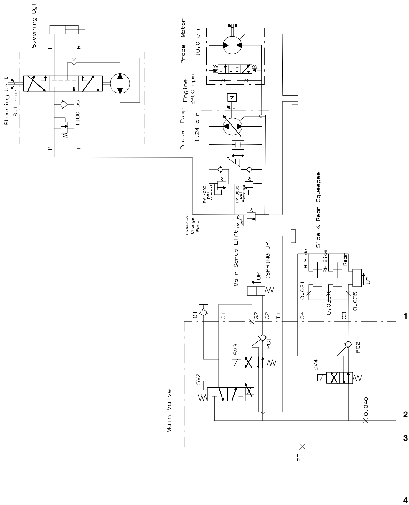
Fig. 61 - Hydraulic Schematic (002283- )
