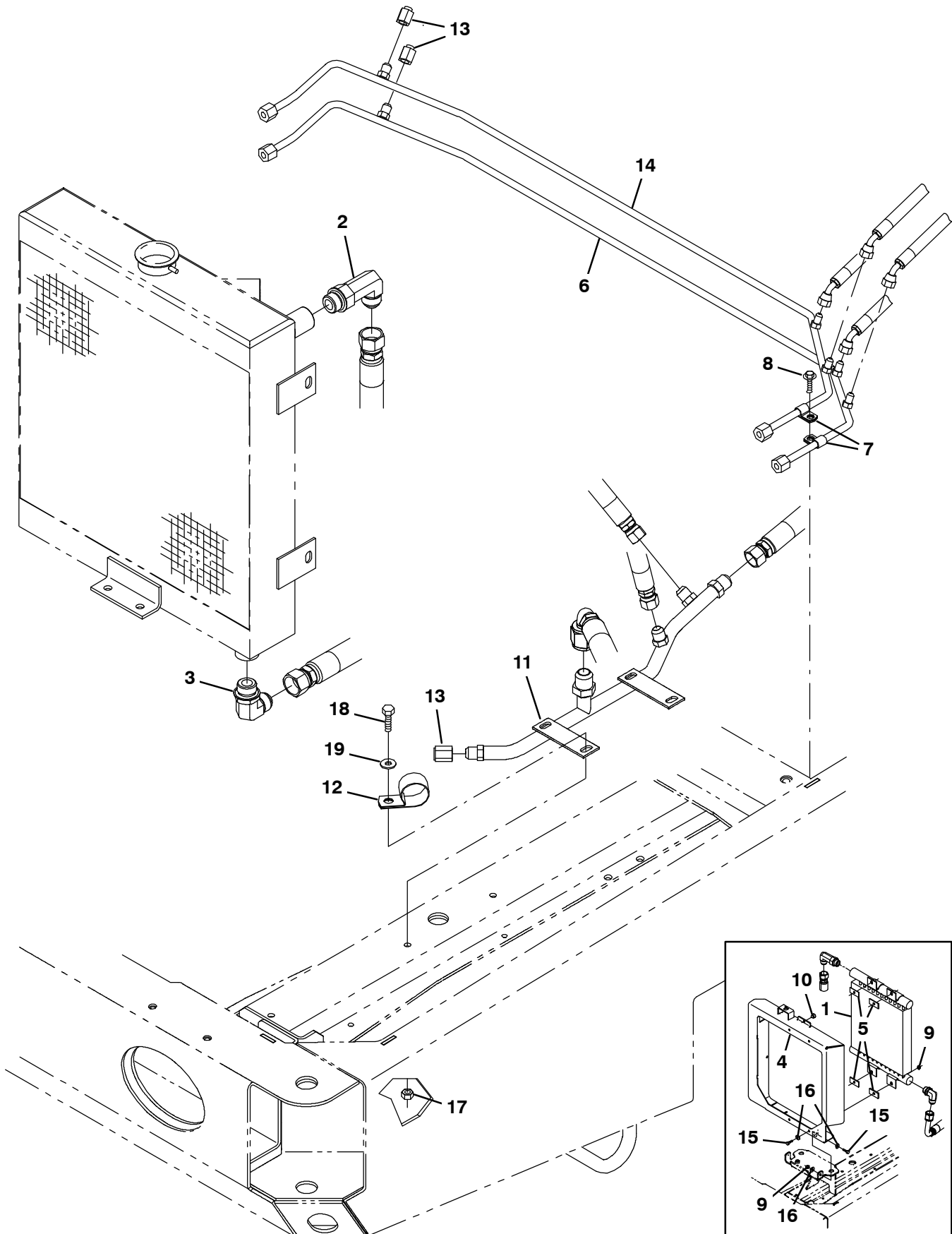
Fig. 68 - Hydraulic Cooler and Tubes Group
