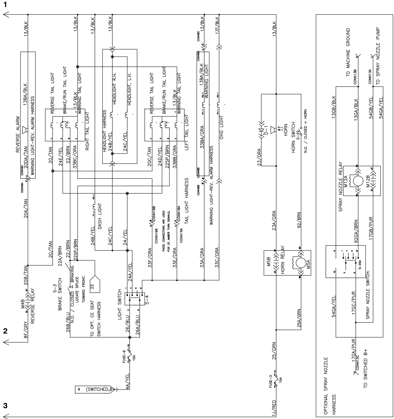
Fig. 73 - Electrical Schematic (001743-
