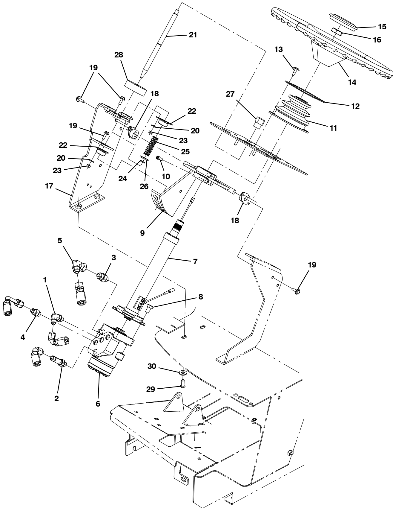
Fig. 8 - Steering Group
