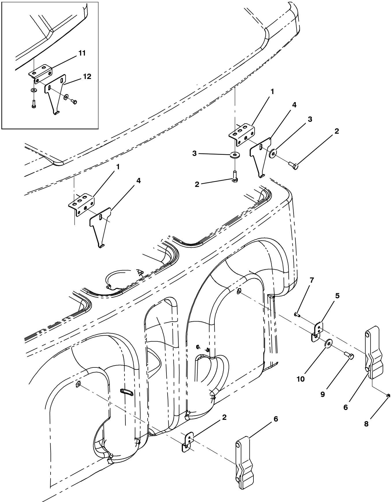
Fig. 42 - Transport Kit
