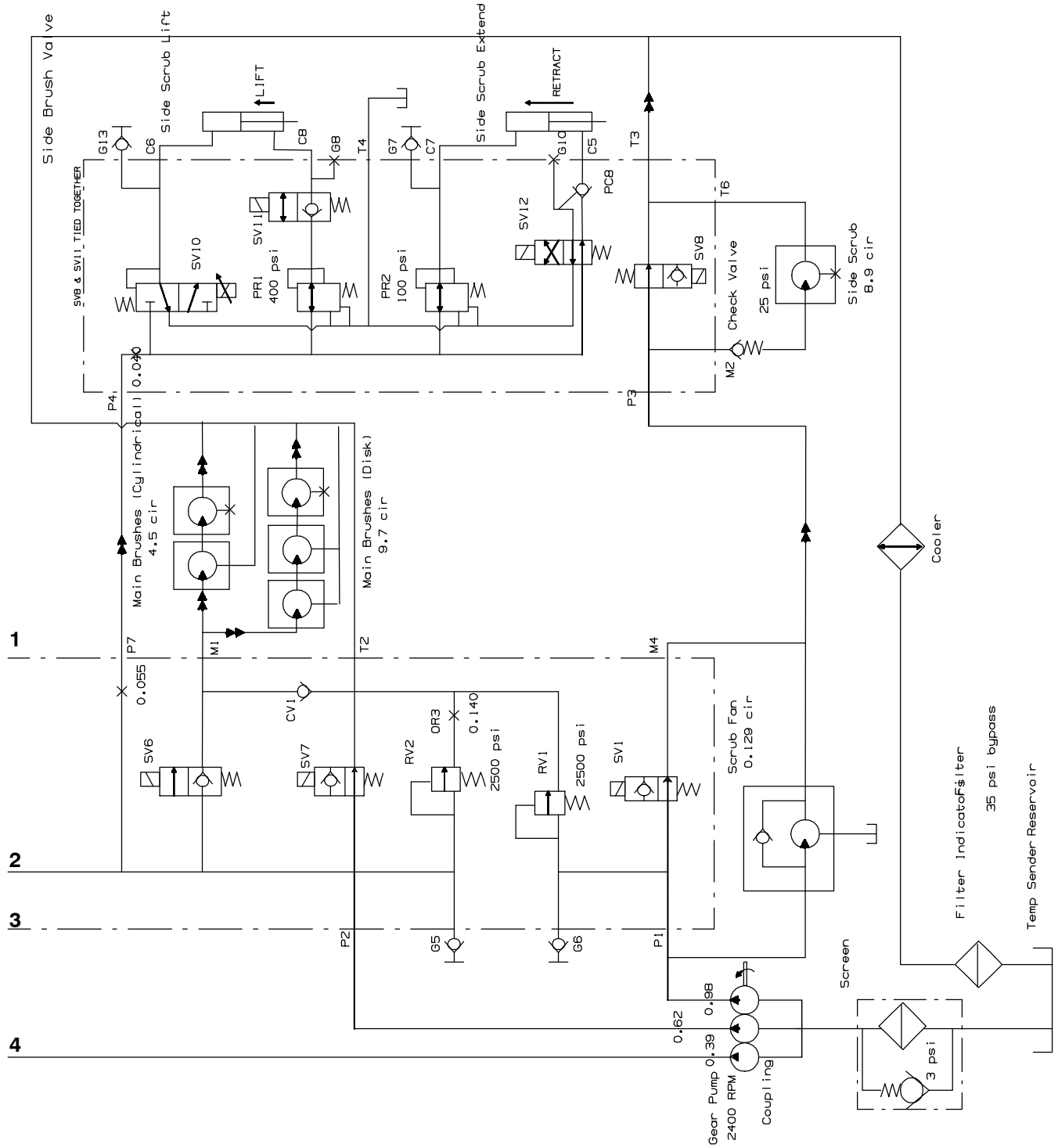
Fig. 60 - Hydraulic Schematic (001504-002282)
