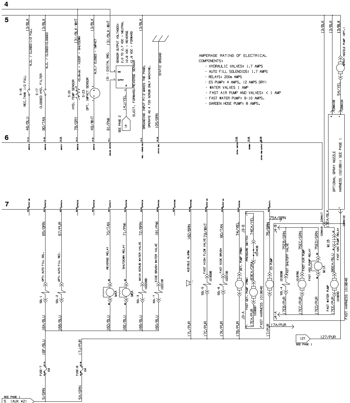
Fig. 72 - Electrical Schematic (001500-001742)
