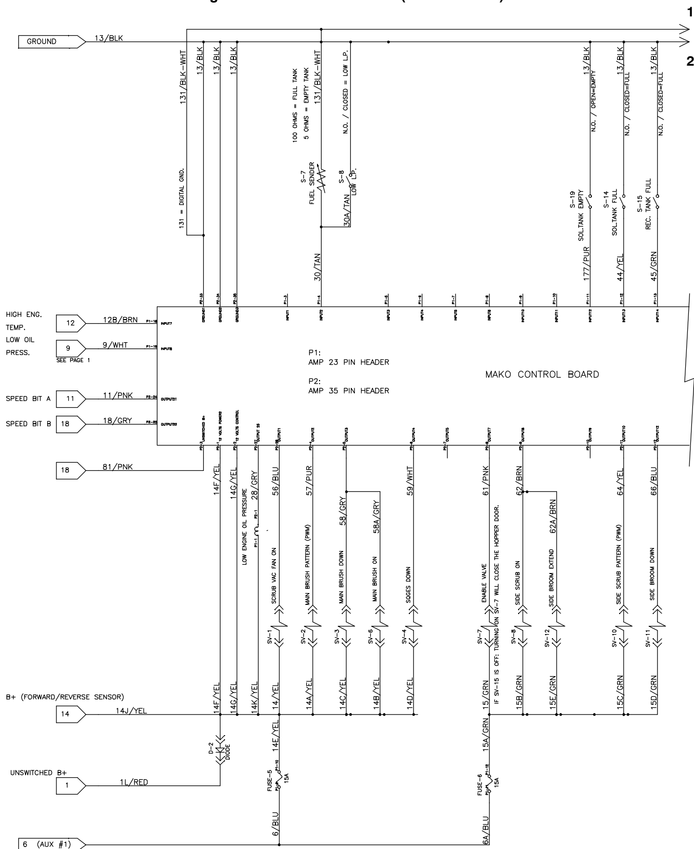
Fig. 73 - Electrical Schematic (001743- )
