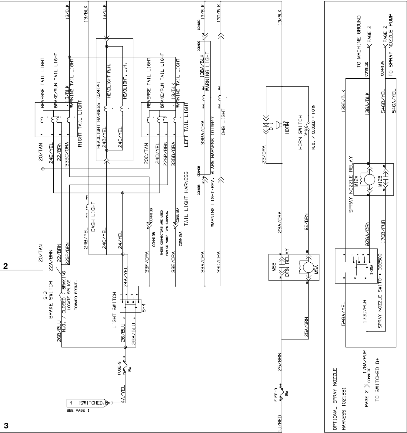
Fig. 72 - Electrical Schematic (001500-001742)
