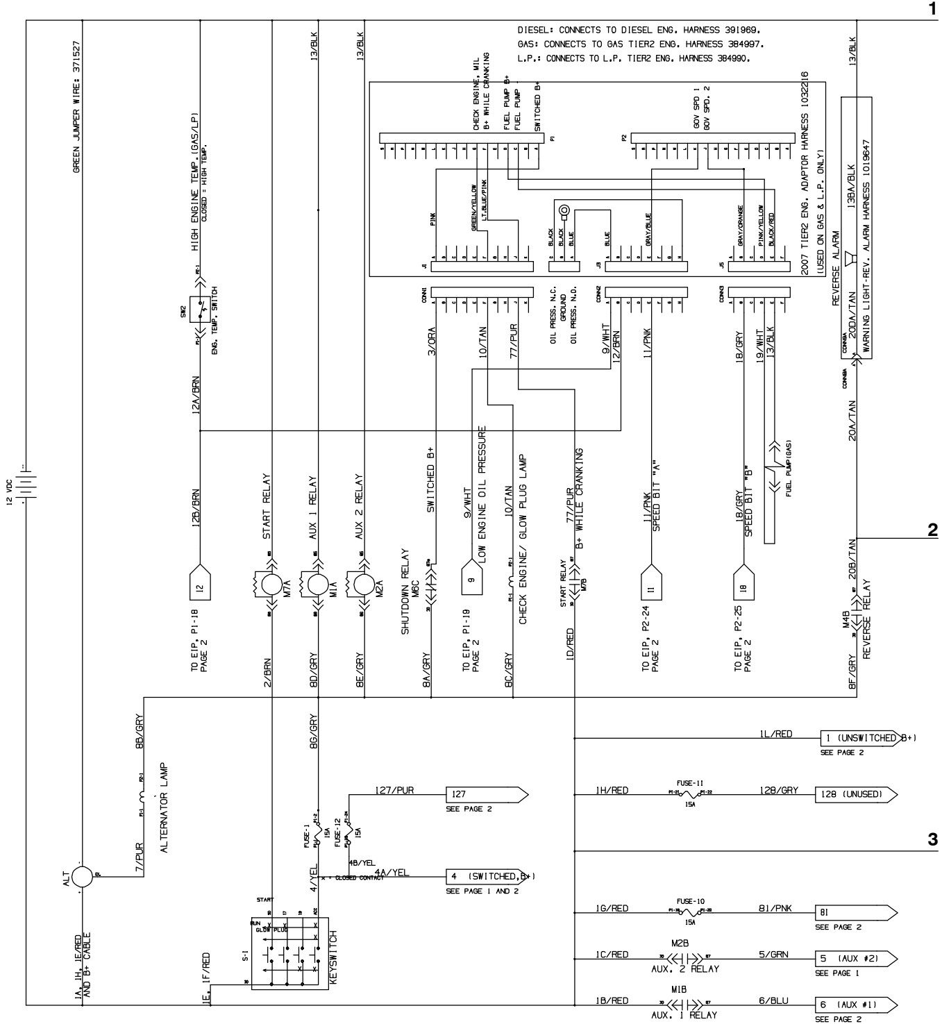
Fig. 72 - Electrical Schematic (001500-001742)
