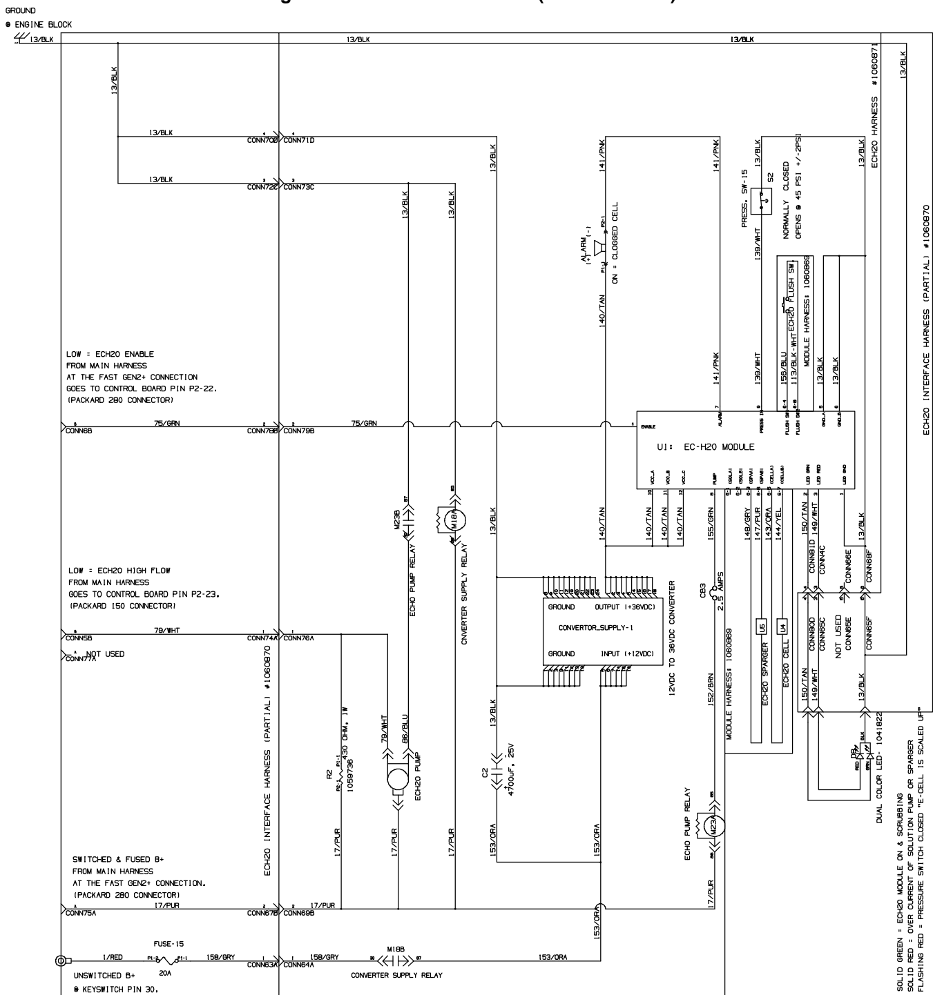
Fig. 73 - Electrical Schematic (001743- )
