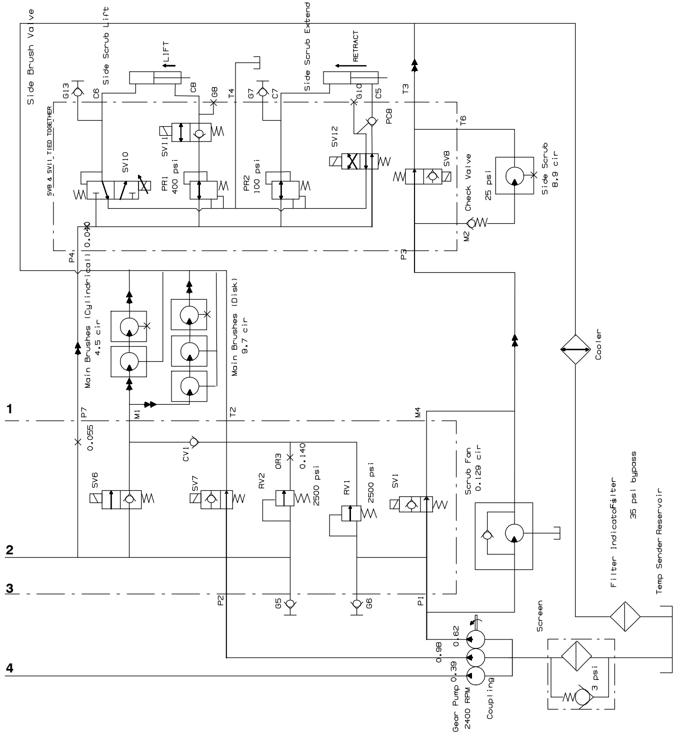
Fig. 61 - Hydraulic Schematic (002283- )
