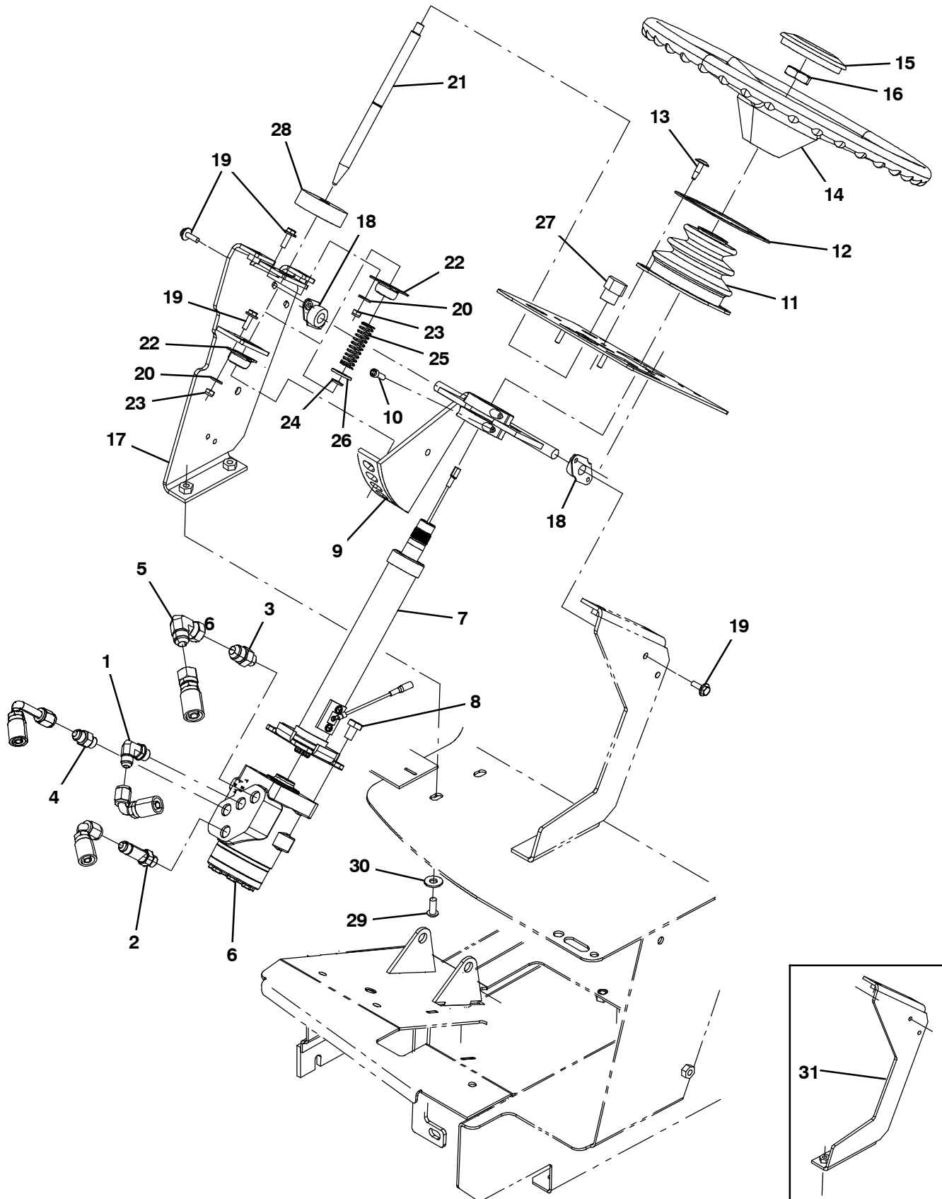
Fig. 8 - Steering Group
