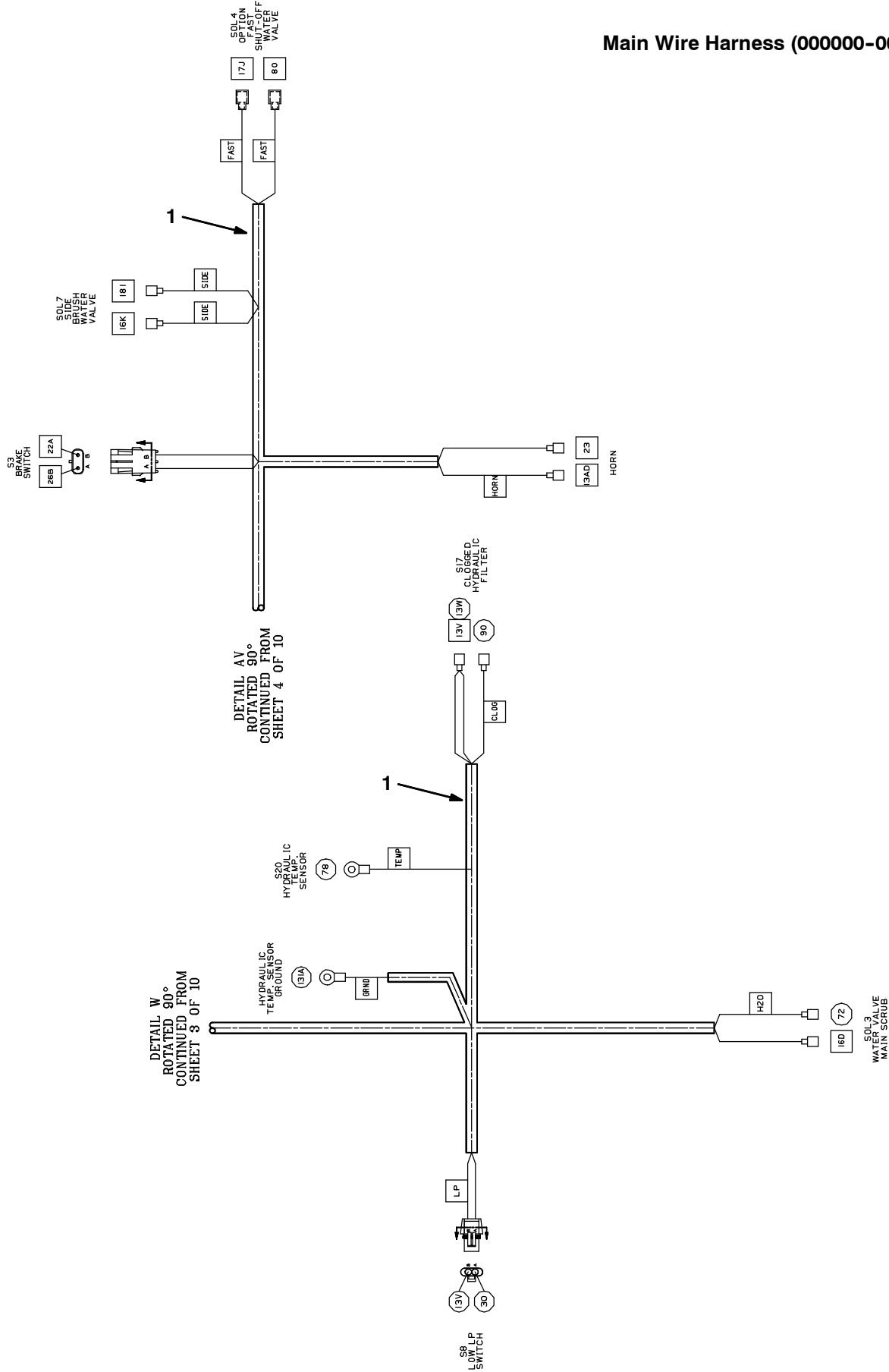
Fig. 81 - Electrical Wire Harnesses Group
