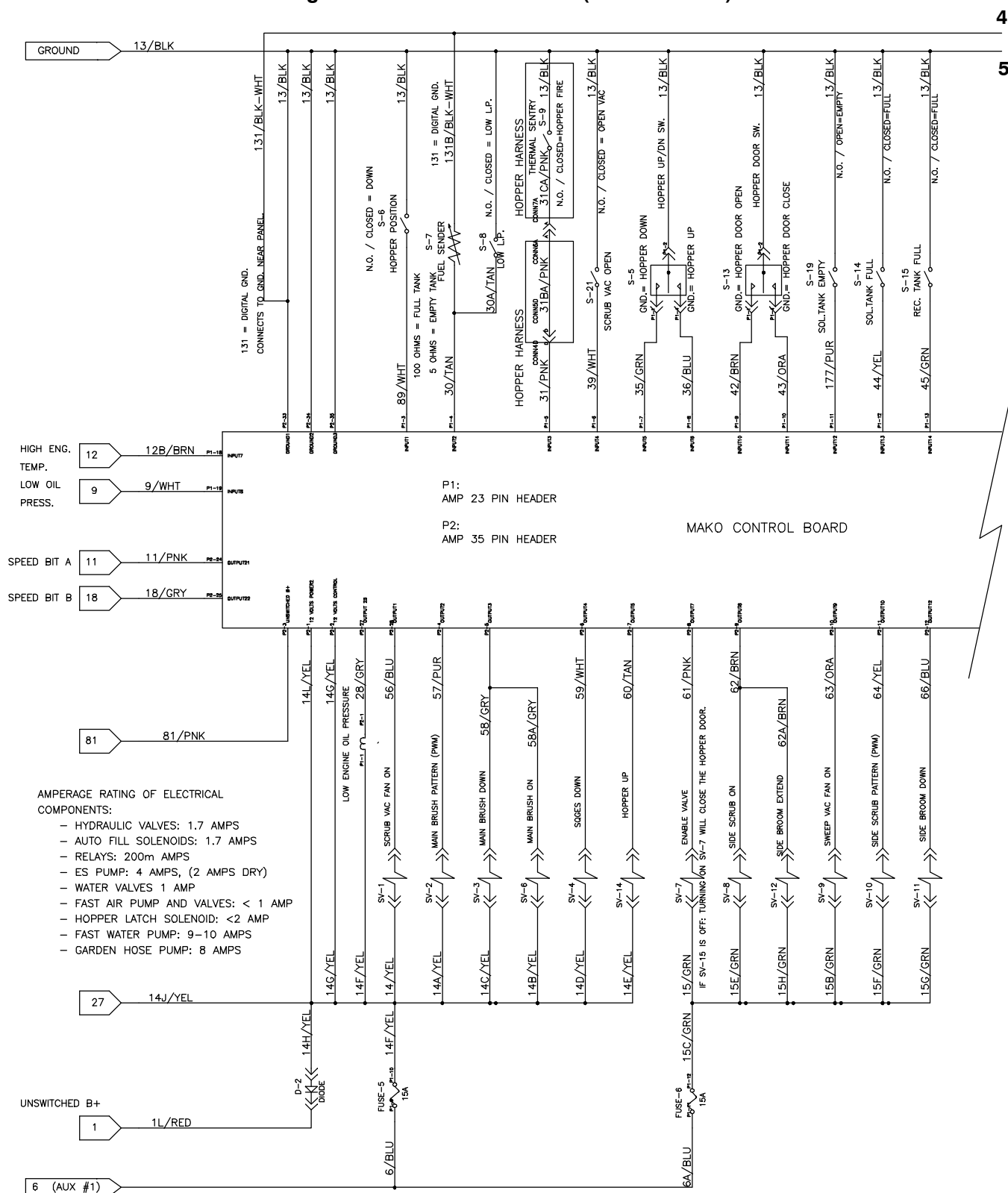
Fig. 75 - Electrical Schematic (002533- )
