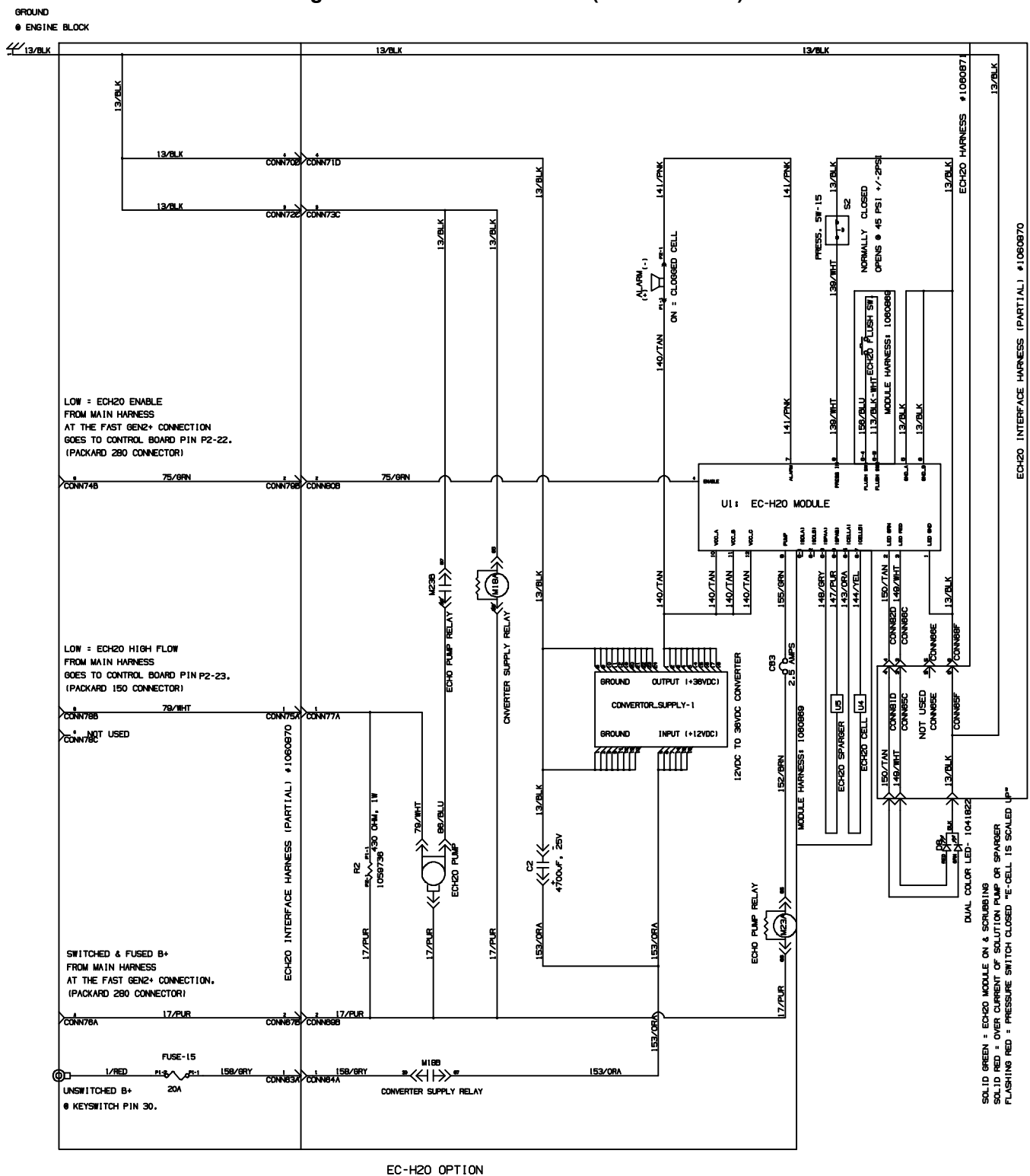
Fig. 75 - Electrical Schematic (002533- )
