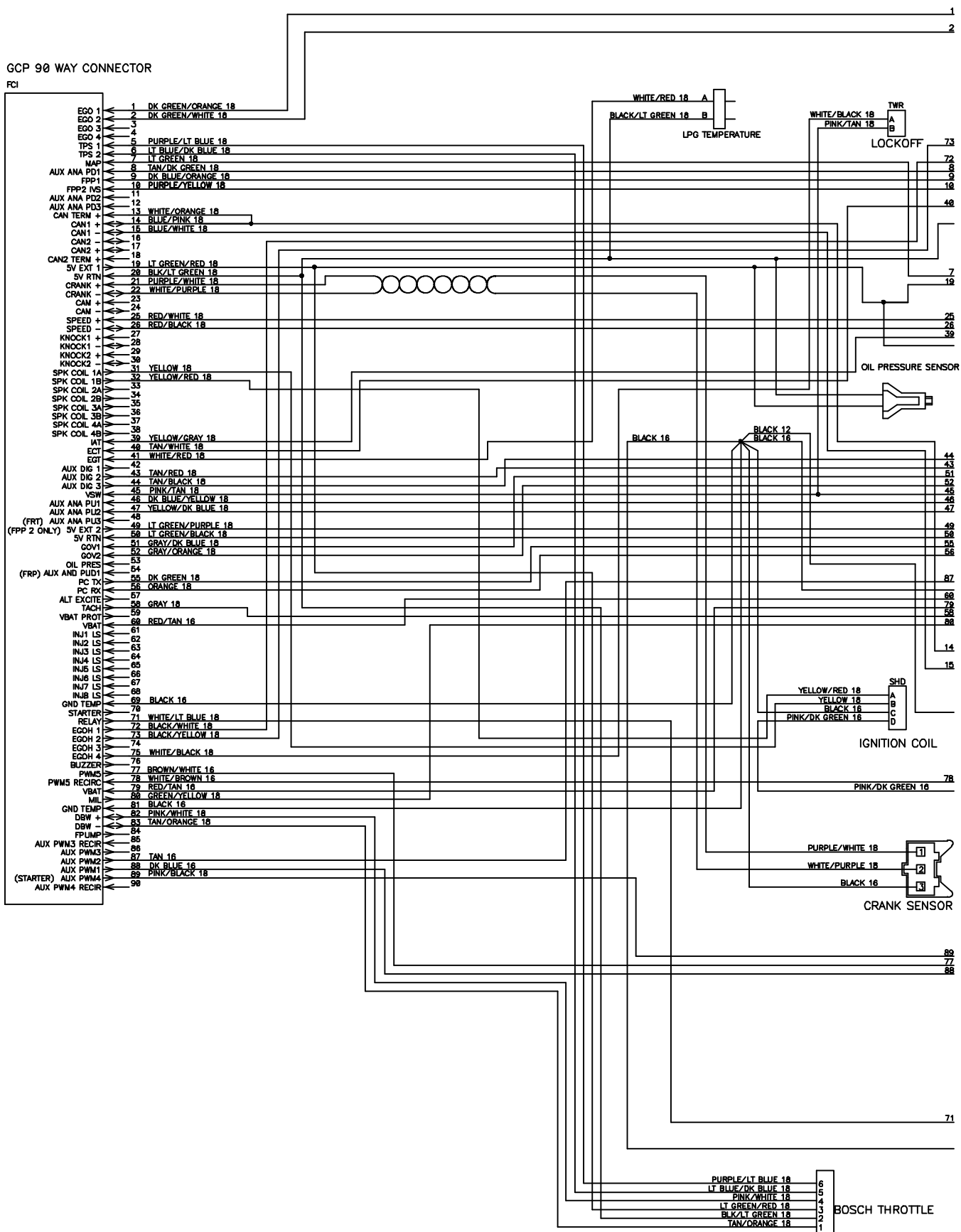
Fig. 80 - Electrical Schematic, LPG Engine Harness (003123- )
