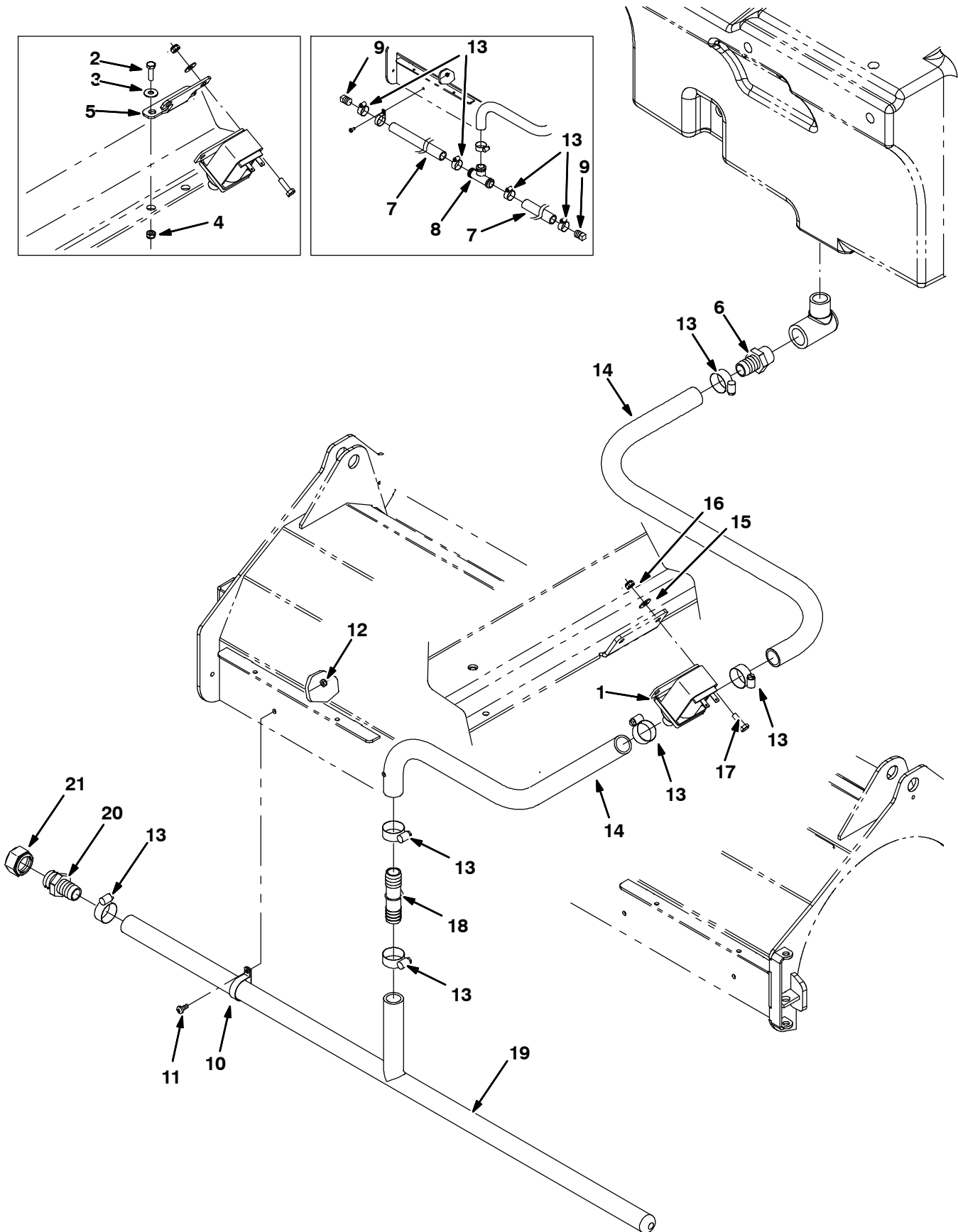
Fig. 56 - Solution Control Group
