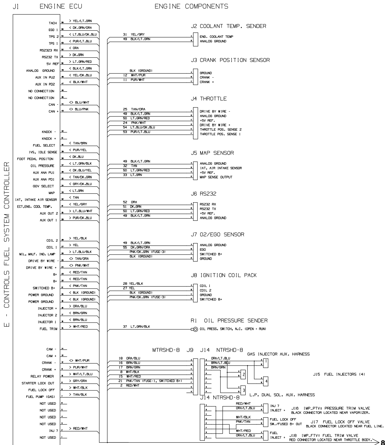
Fig. 76 - Electrical Schematic, Gas/LPG Engine Harness (000000-001999)
