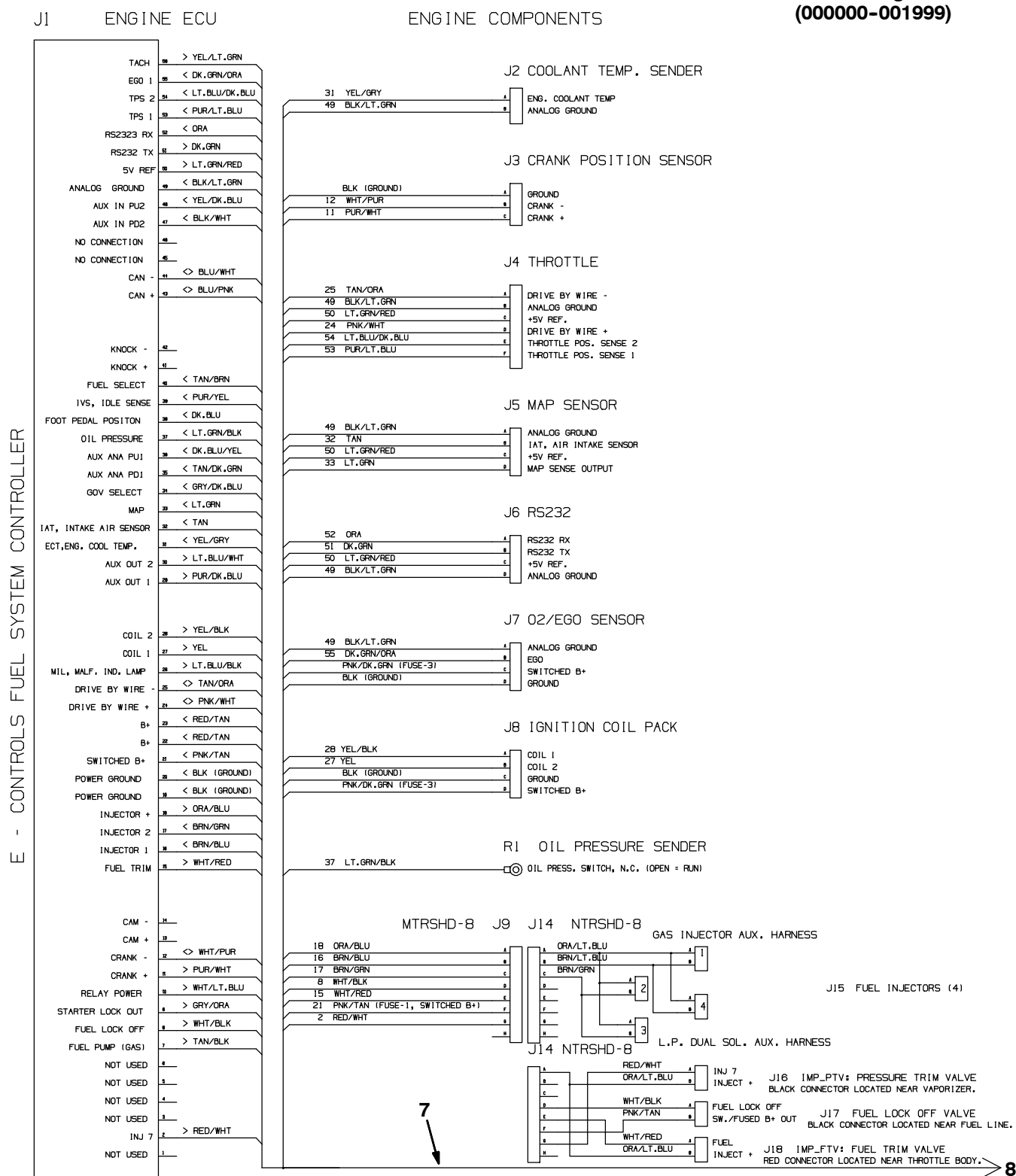
Fig. 81 - Electrical Wire Harnesses Group
