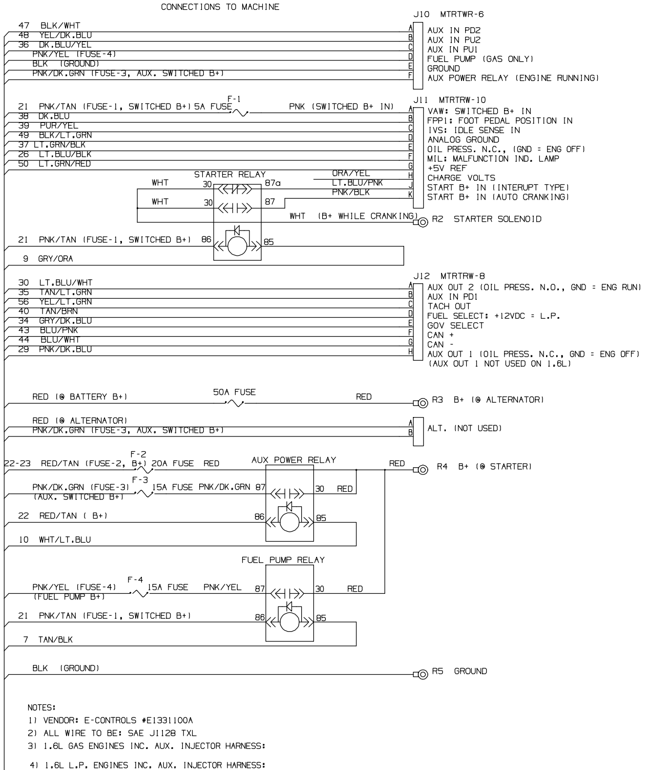
Fig. 76 - Electrical Schematic, Gas/LPG Engine Harness (000000-001999)
