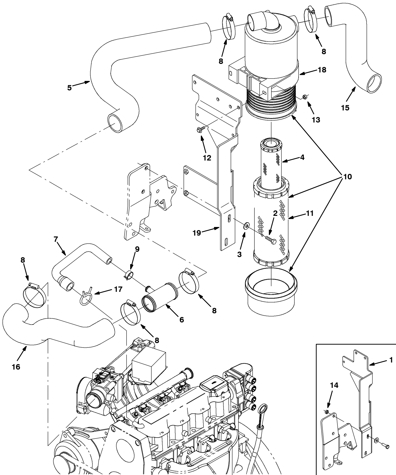
Fig. 23 - Engine Air Cleaner Group, Gasoline (002000- )
