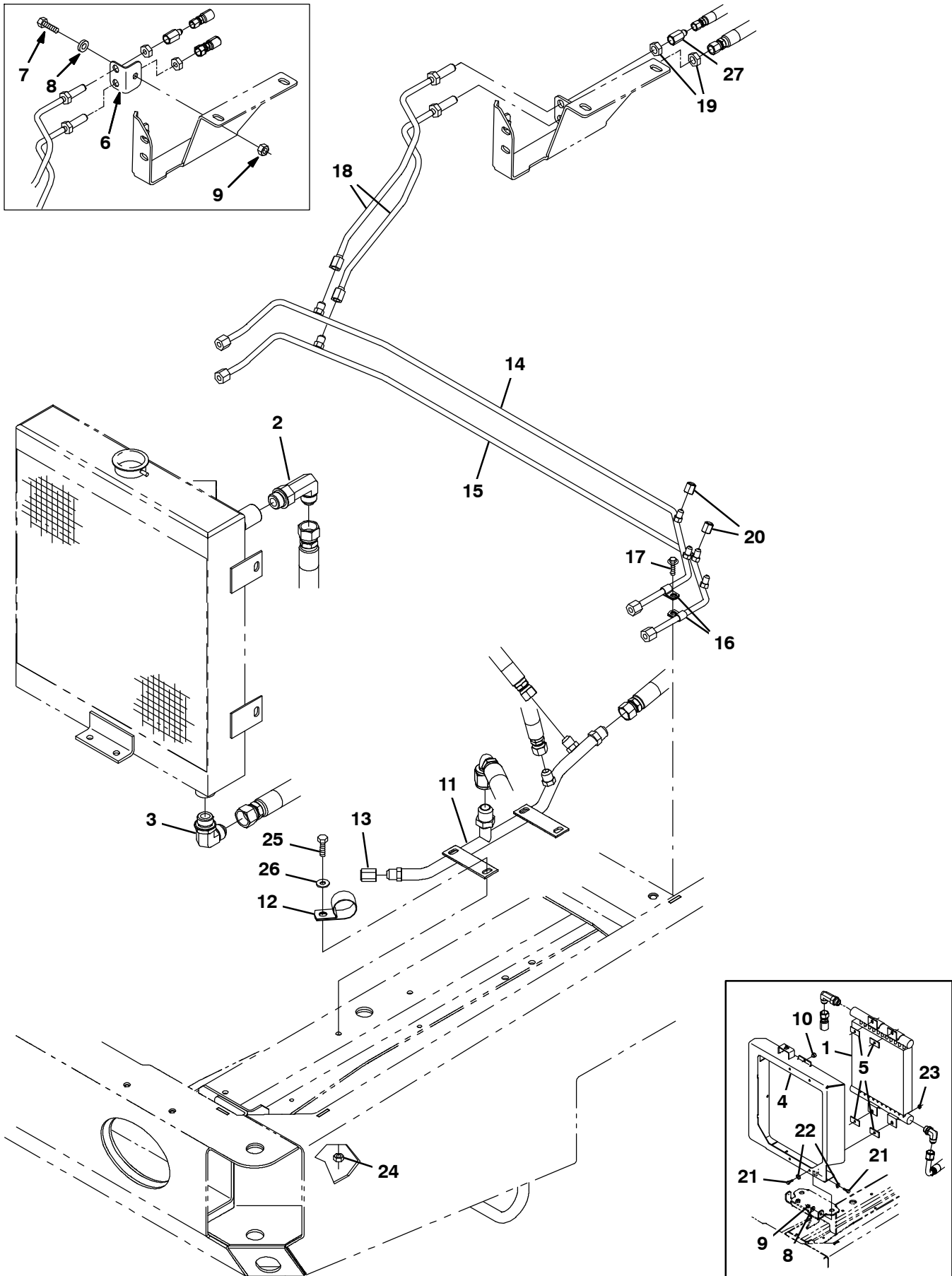
Fig. 69 - Hydraulic Cooler and Tubes Group
