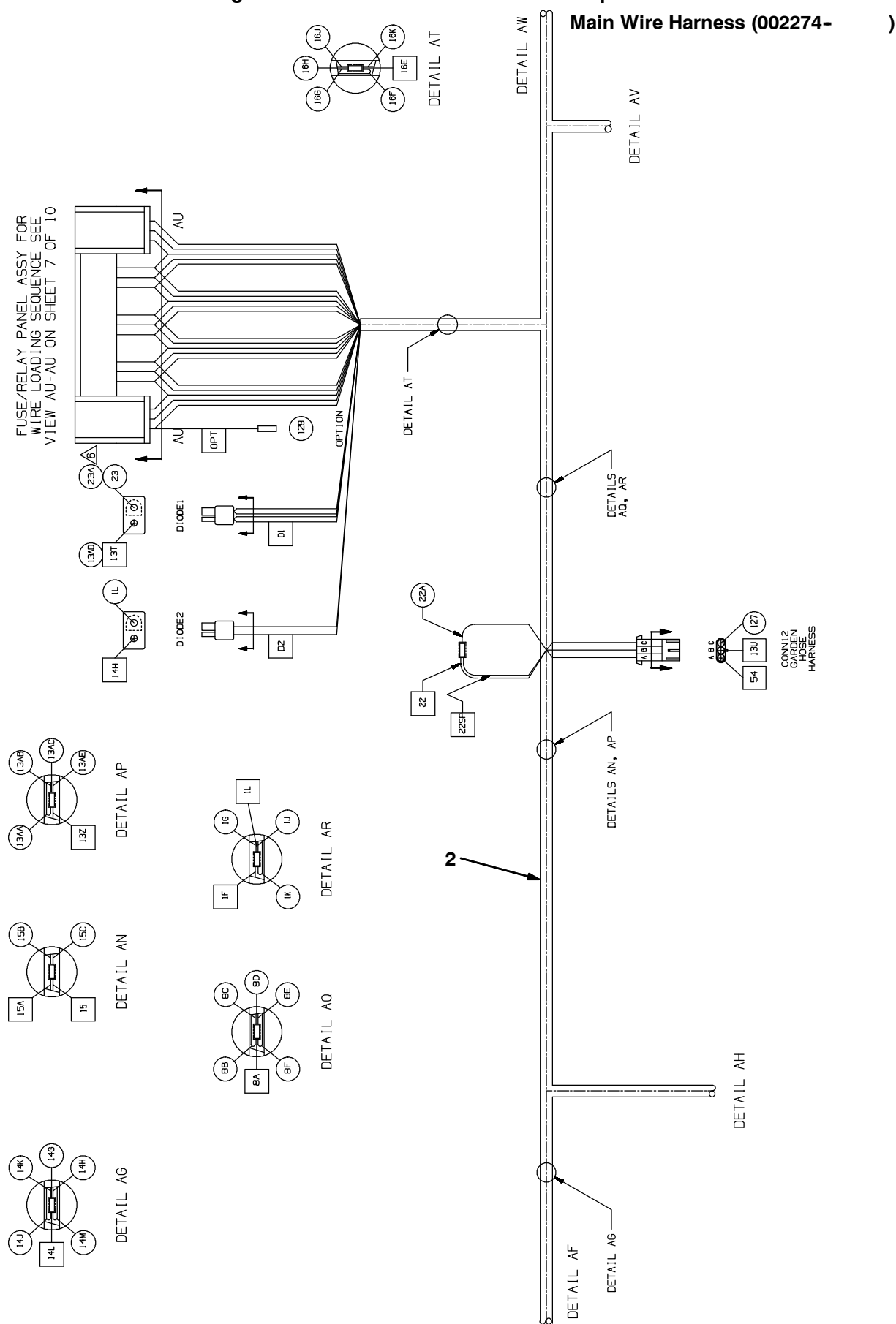
Fig. 81 - Electrical Wire Harnesses Group
