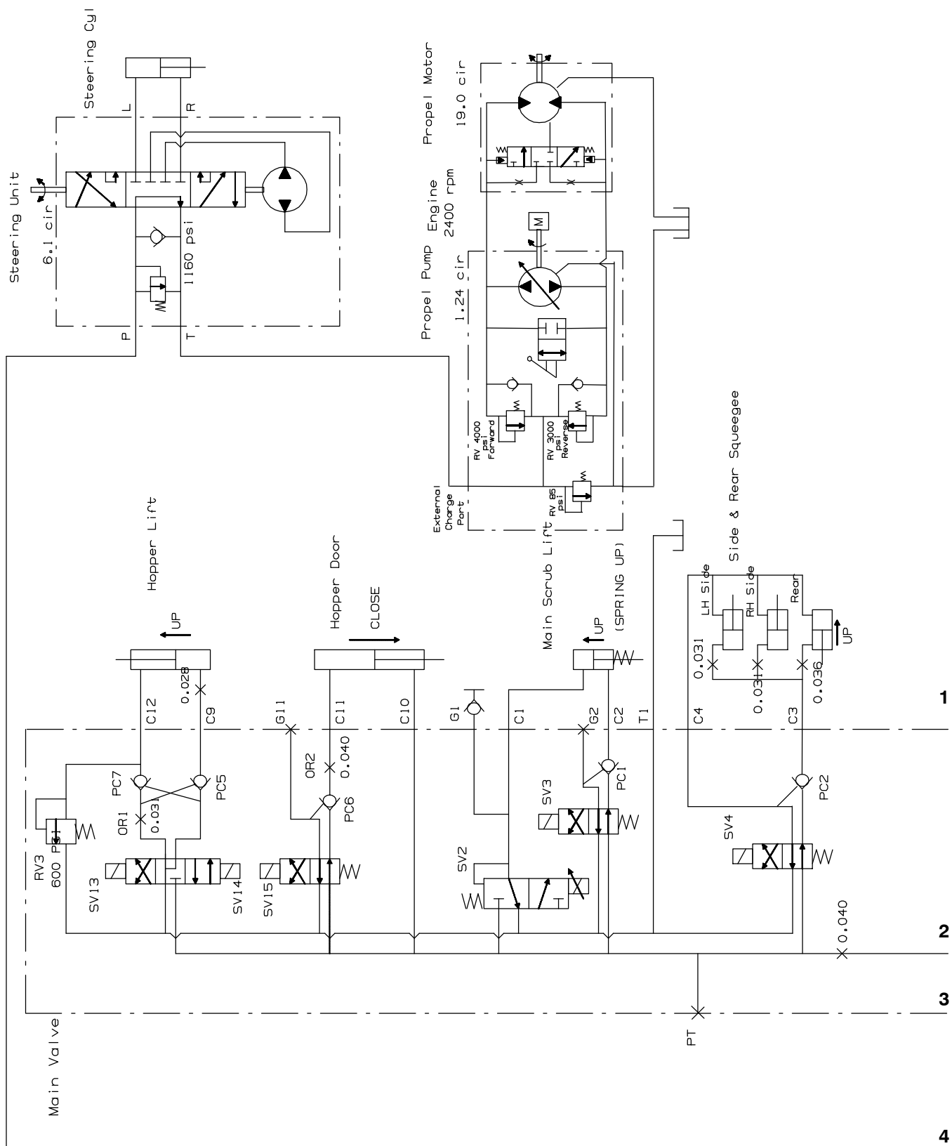
Fig. 63 - Hydraulic Schematic (003298- )
