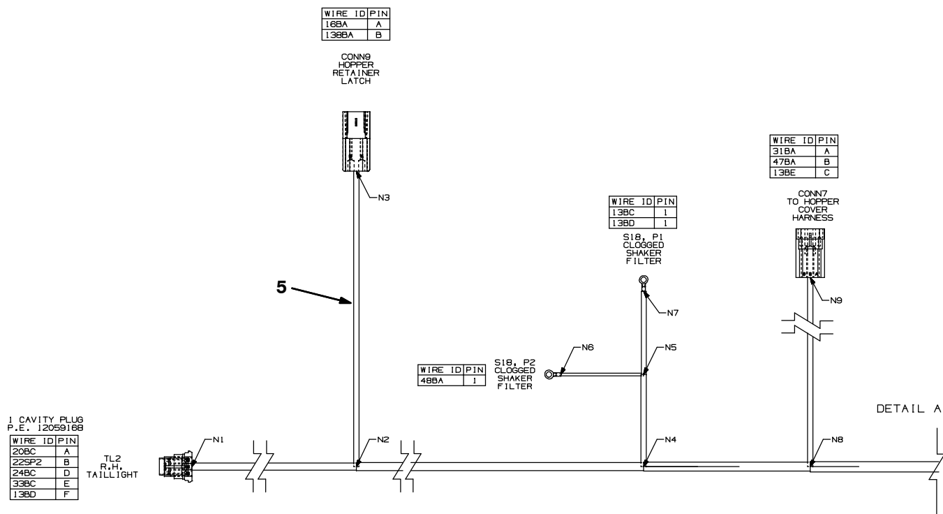
Fig. 81 - Electrical Wire Harness Group
