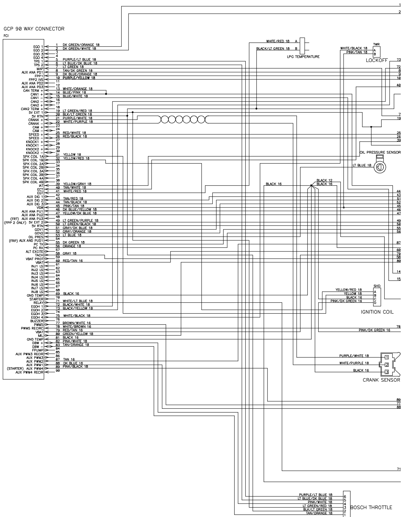
Fig. 79 - Electrical Schematic, LPG Engine Harness (002000-003122)
