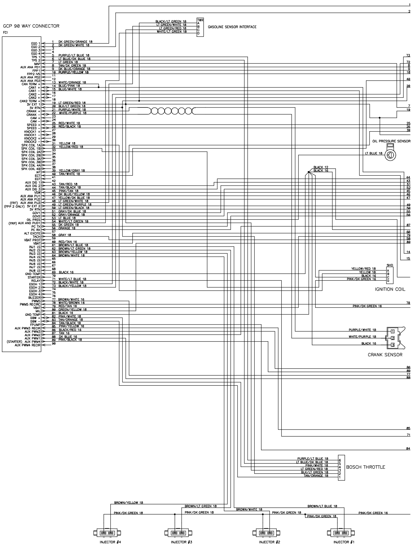
Fig. 77 - Electrical Schematic, Gas Engine Harness (002000-003122)
