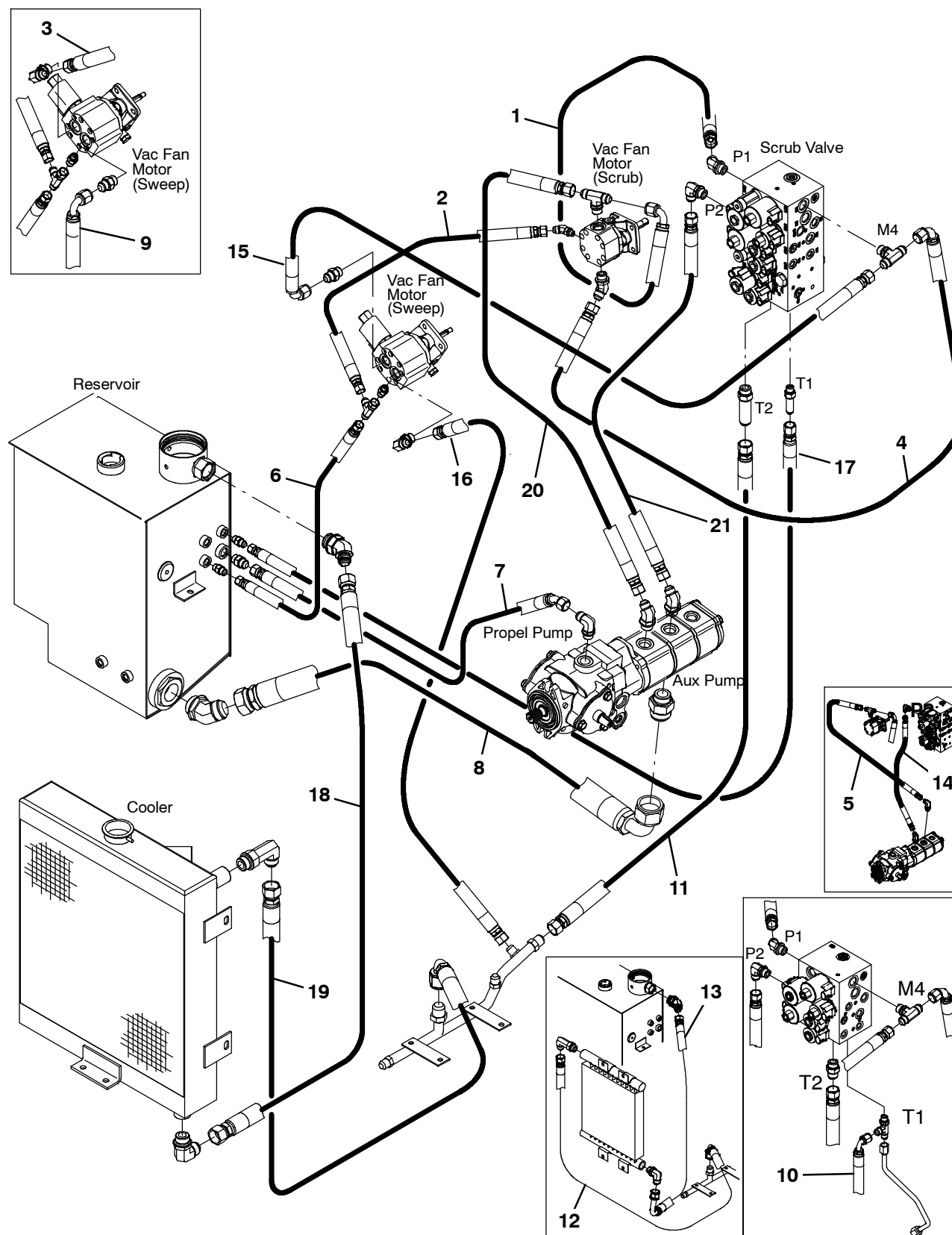
Fig. 65 - Hydraulic Hose Group, Pump and Vacuum Fans
