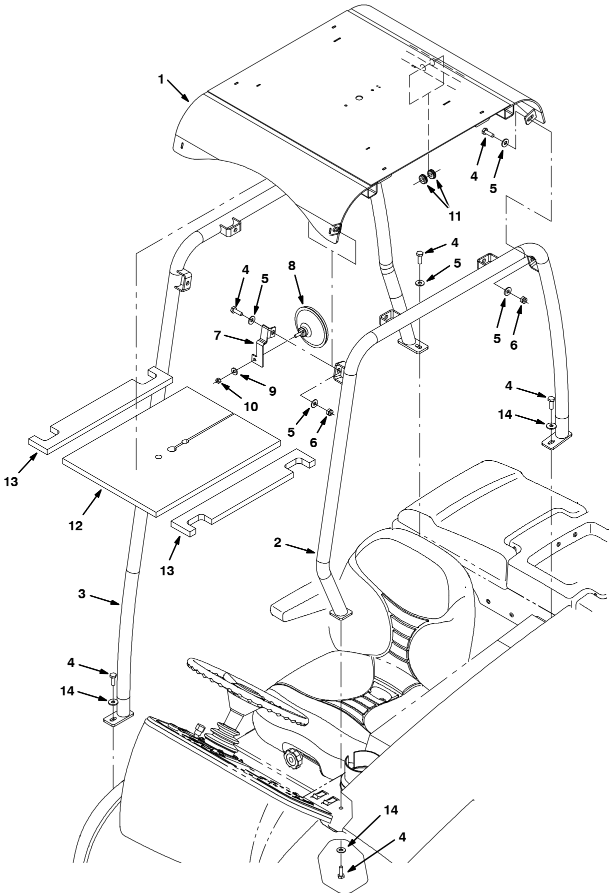
Fig. 28 - Overhead Guard Kit
