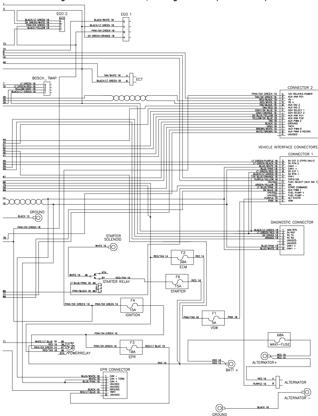
Fig. 79 - Electrical Schematic, LPG Engine Harness (002000-003122)
