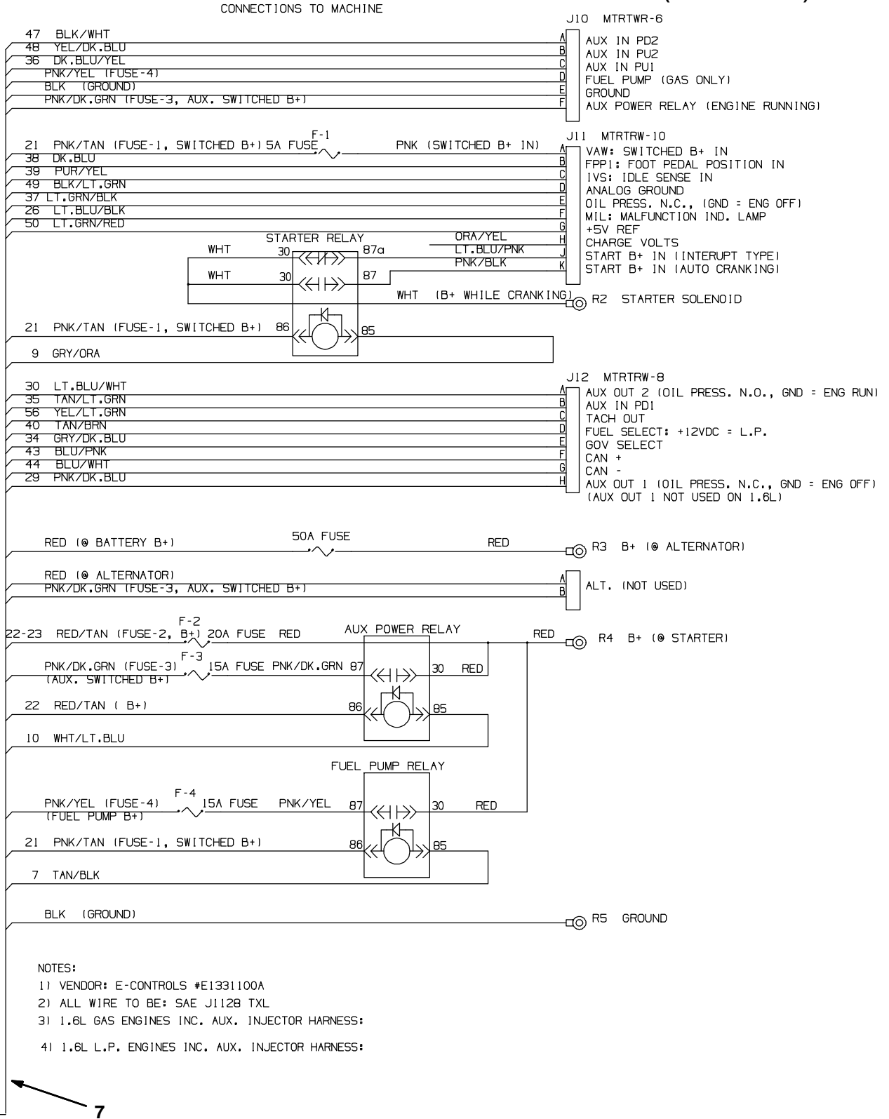
Fig. 81 - Electrical Wire Harnesses Group
