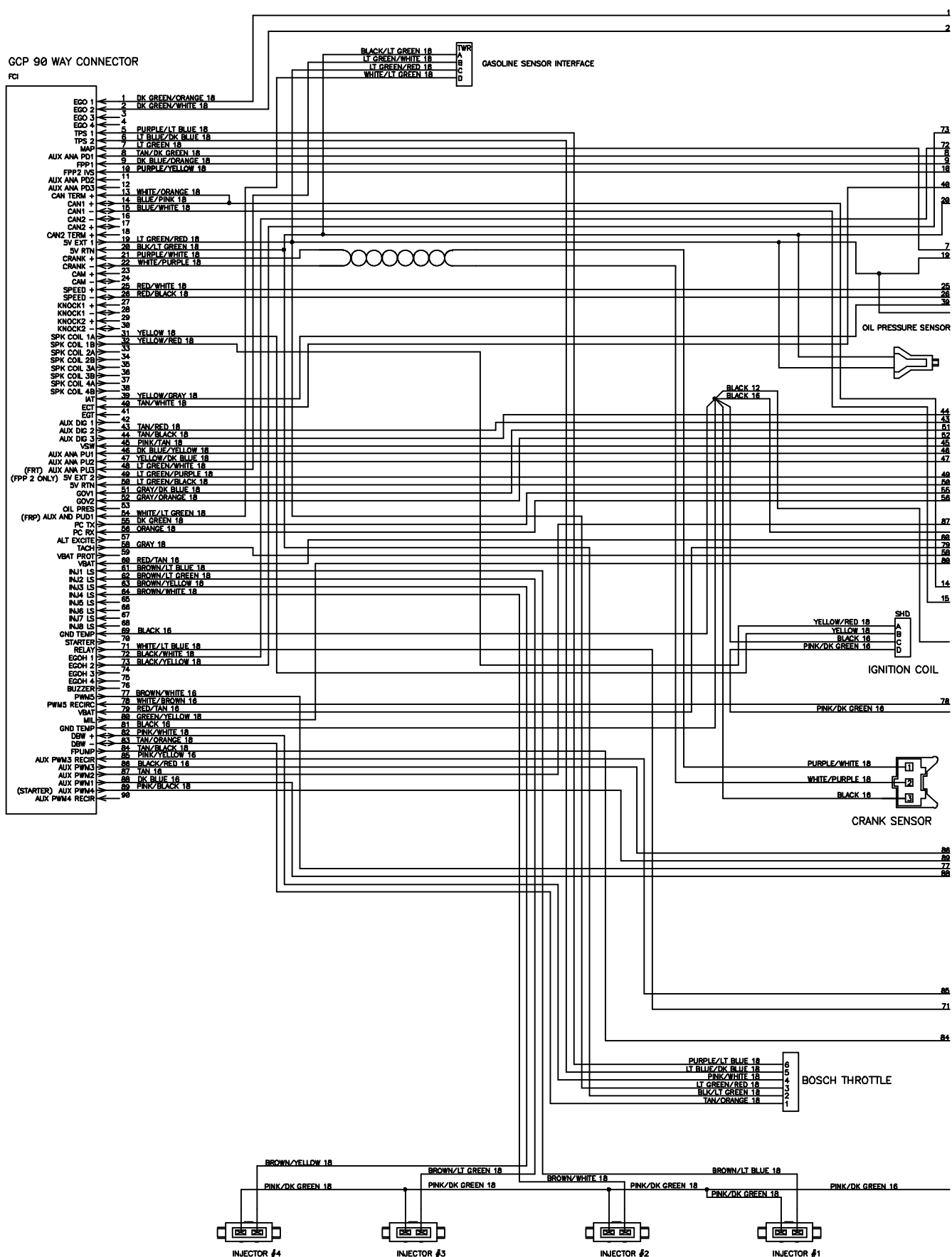
Fig. 78 - Electrical Schematic, Gas Engine Harness (003123- )
