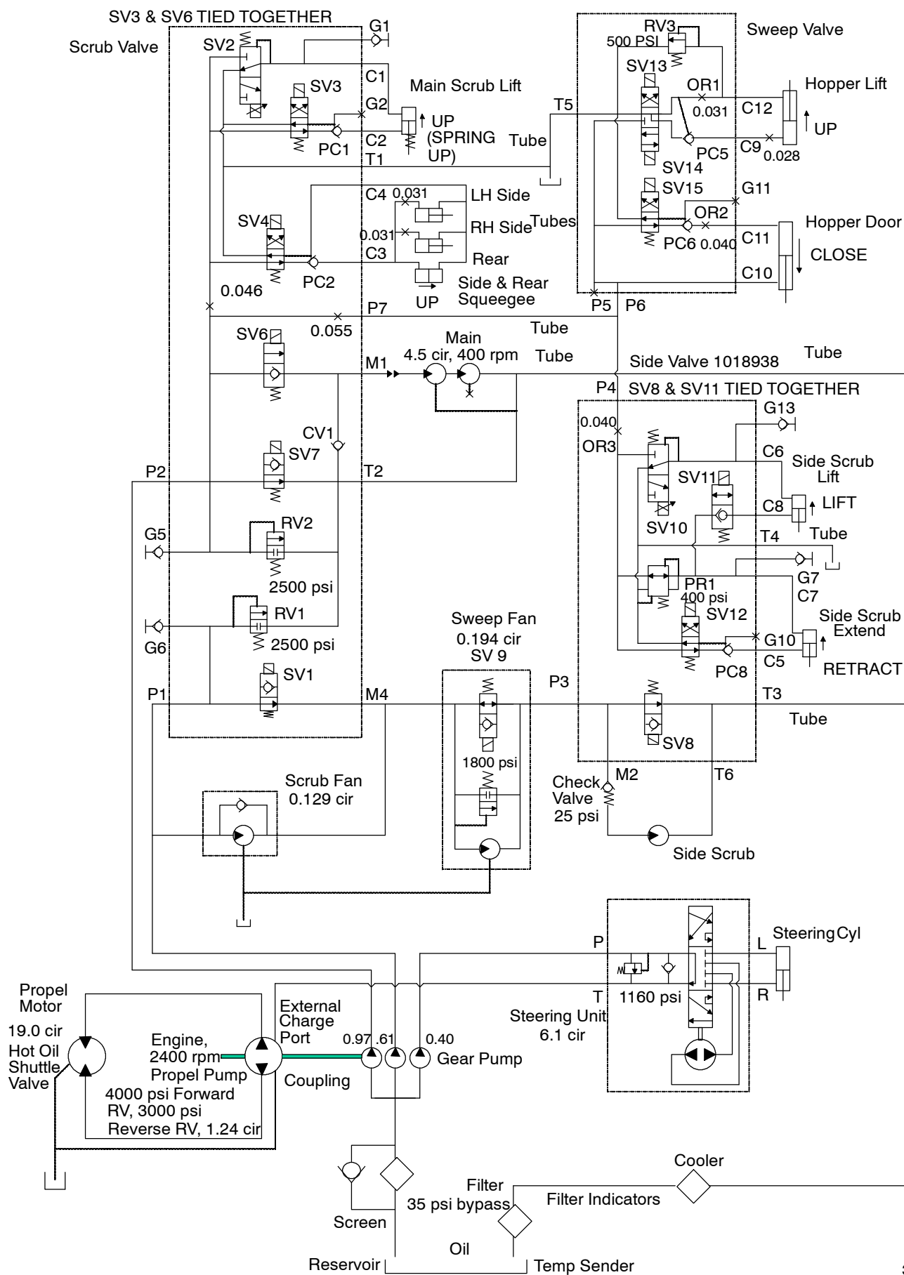
Fig. 61 - Hydraulic Schematic (000000-002699)
