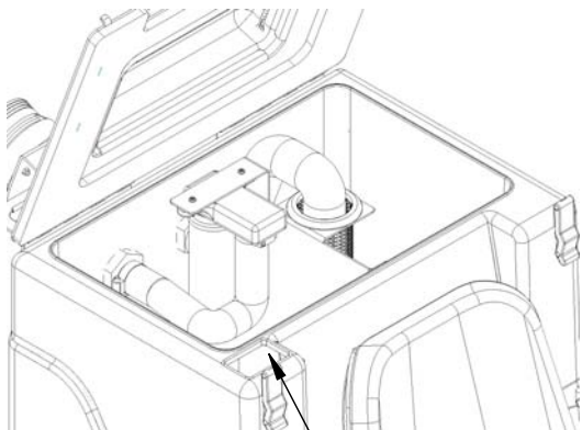
Solution Fill Port
