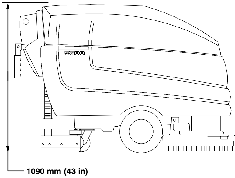
MACHINE DIMENSIONS
